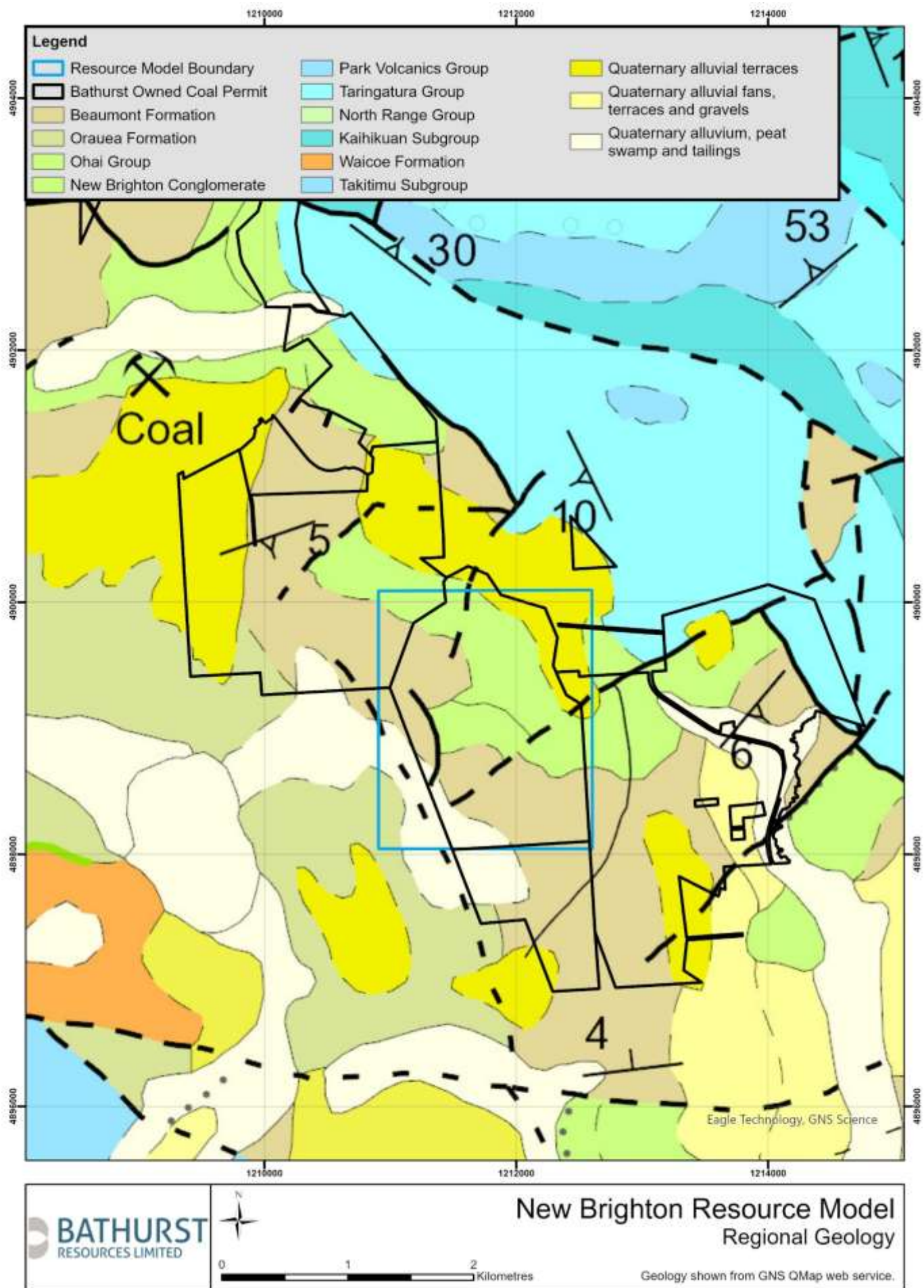
Figure 2: Regional Geology
