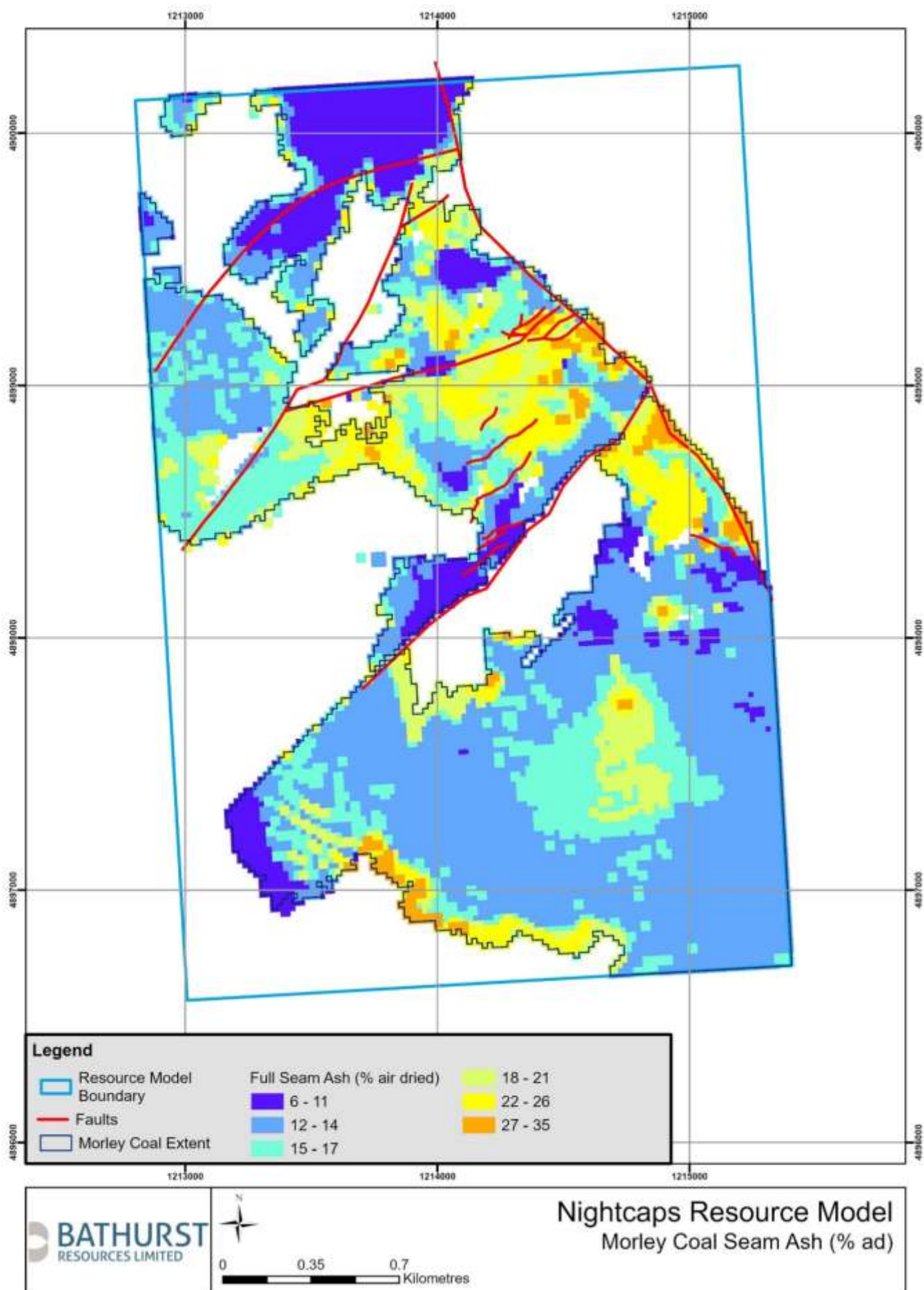
Figure 21: Morley Formation full seam air dried ash distribution
