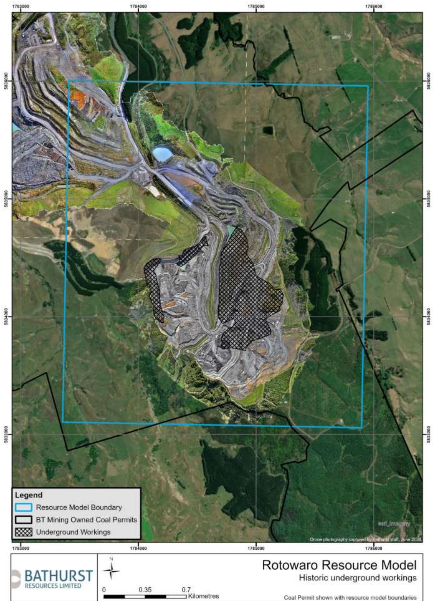
Figure 6: Plan showing the extent of remaining Underground Workings
