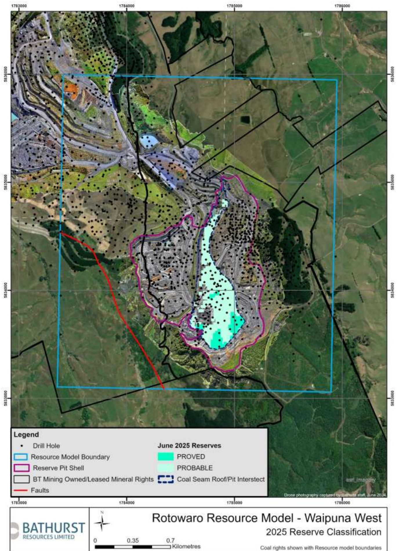
Figure 8: Plan showing the reserve classification for the Taupiri Main seam at Waipuna West
