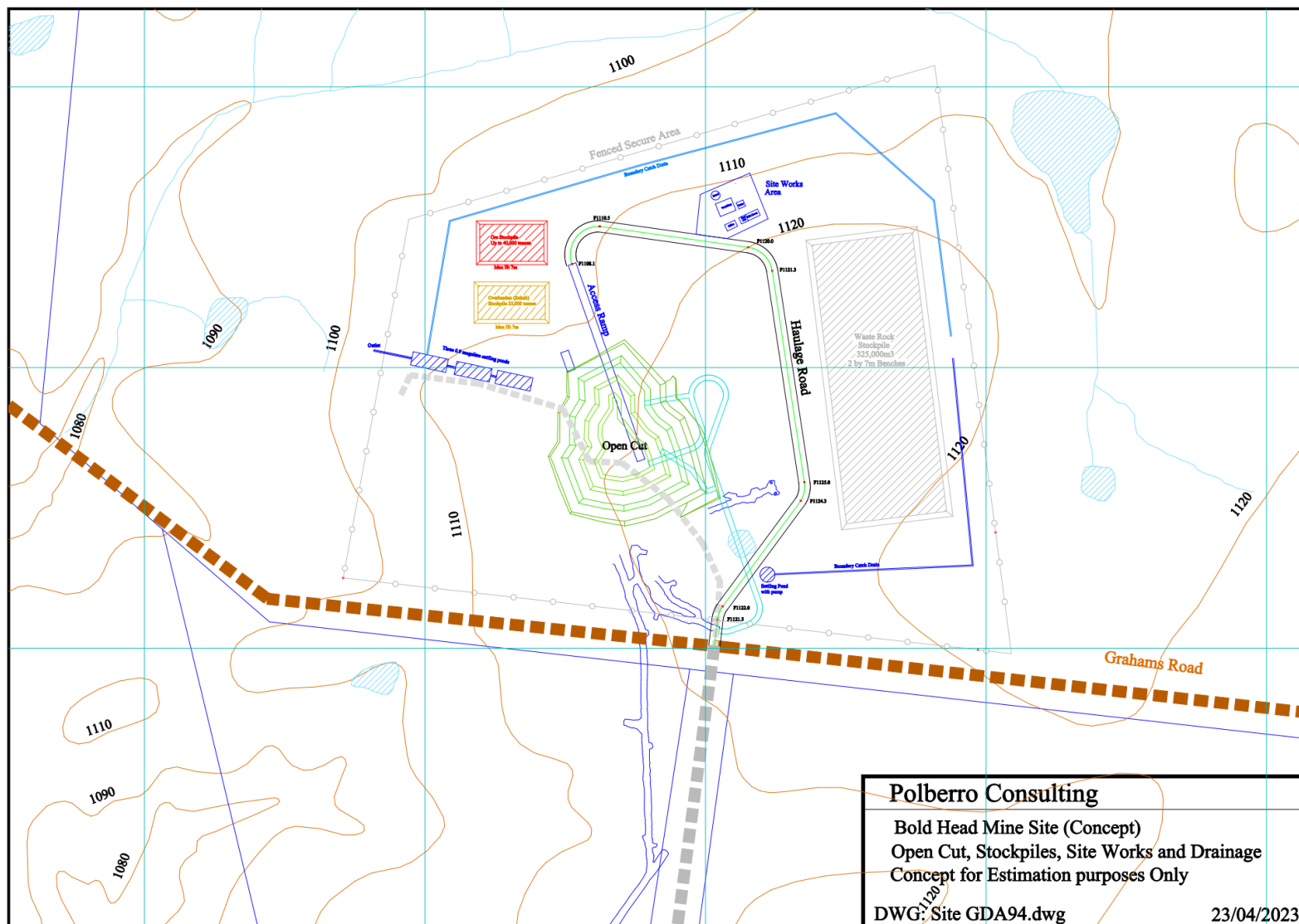
Figure 4. KIS Bold Head Proposed Mine Layout.
