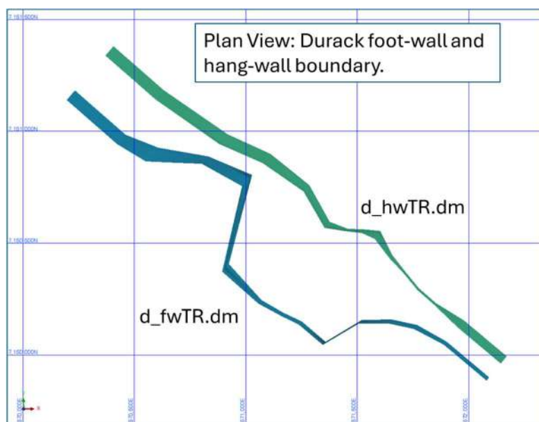
Figure 14-33 Durack footwall and hangingwall boundary. Source: Westgold.
