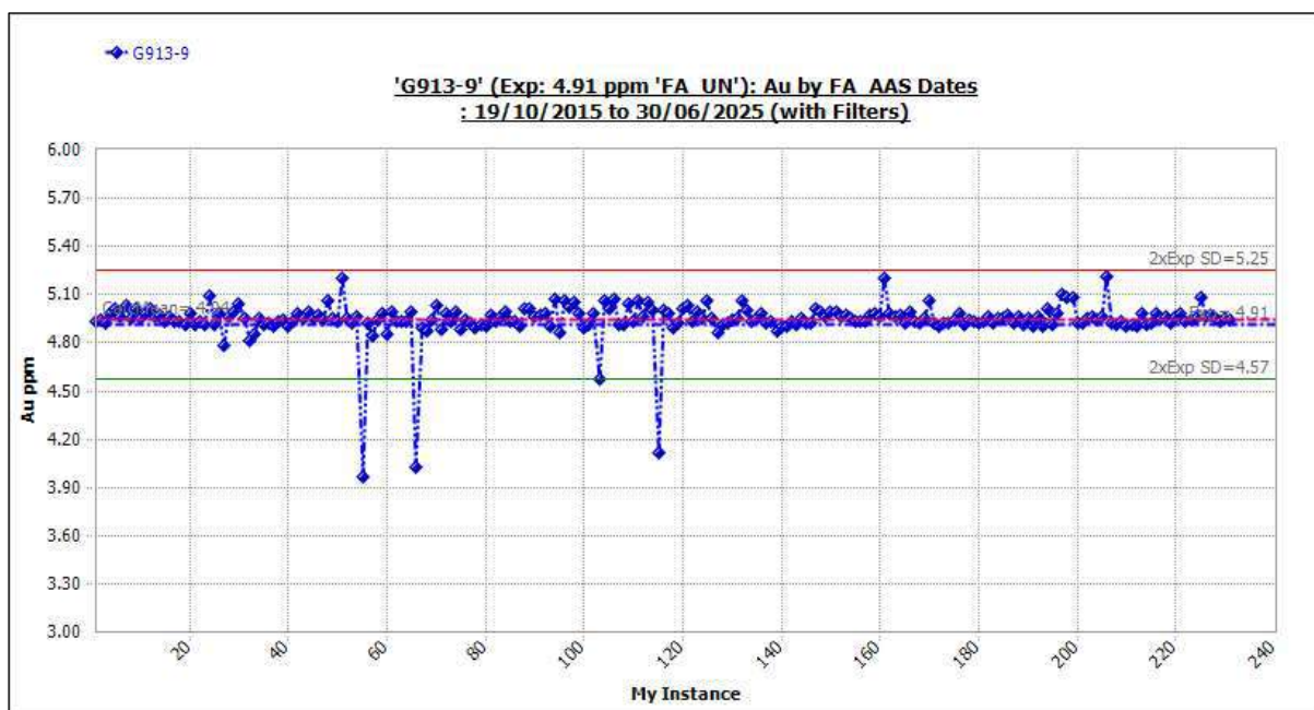
Figure 11-38 Standard G913-9: Outliers Included.
