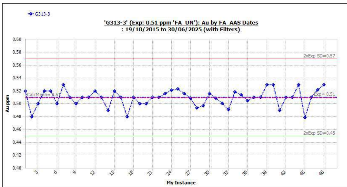
Figure 11-10 Standard G313-3: Outliers Included.
