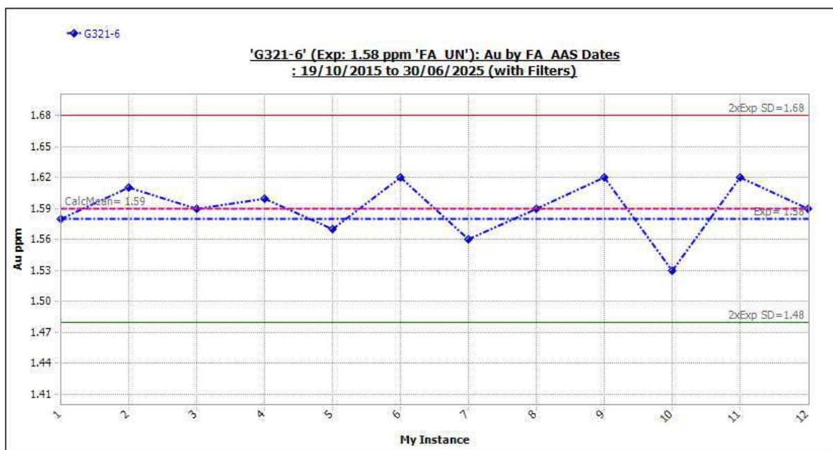
Figure 11-27 Standard G321-6: Outliers Included.
