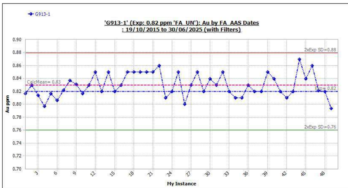
Figure 11-37 Standard G913-1: Outliers Included.
