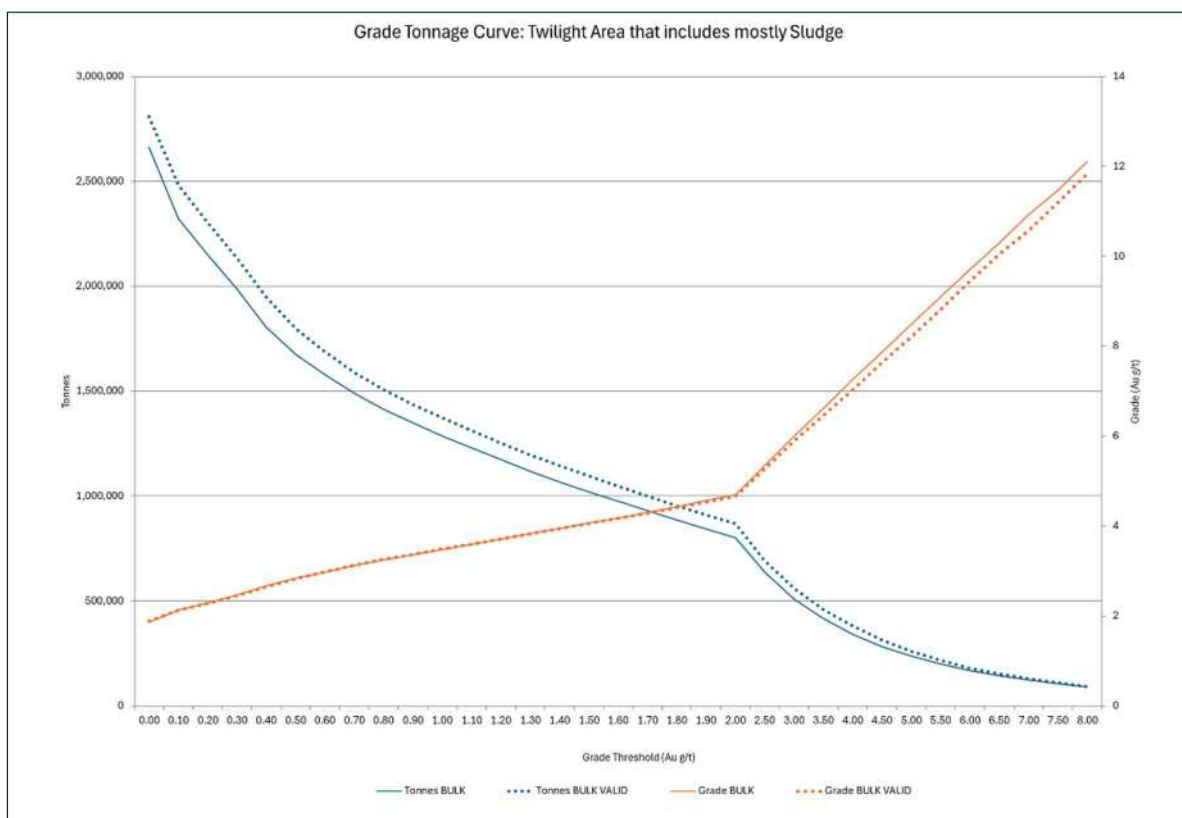
Figure 14-24 Grade tonnage curve comparison showing estimate with and without sludge drilling - Source: Westgold.
