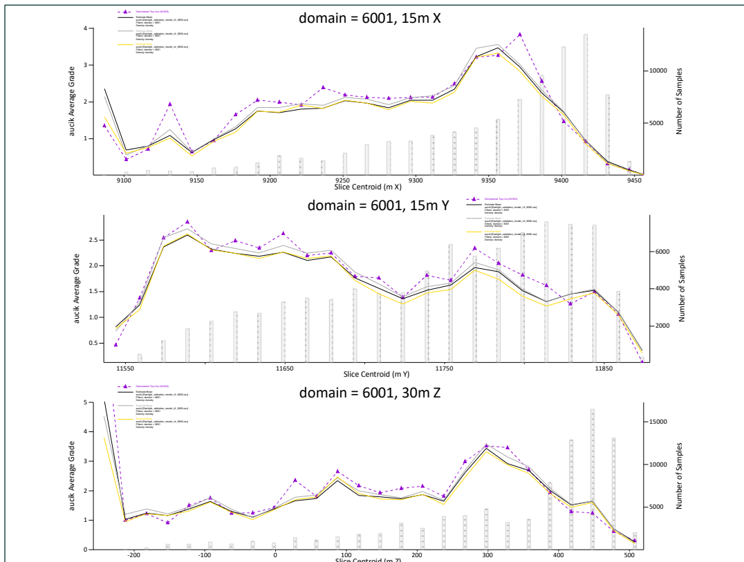
Figure 14-19 Domain 6001 model validation swath plots -Source: Westgold.
