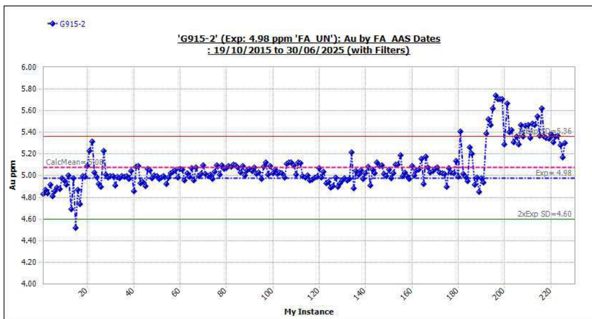
Figure 11-43 Standard G915-2: Outliers Included.
