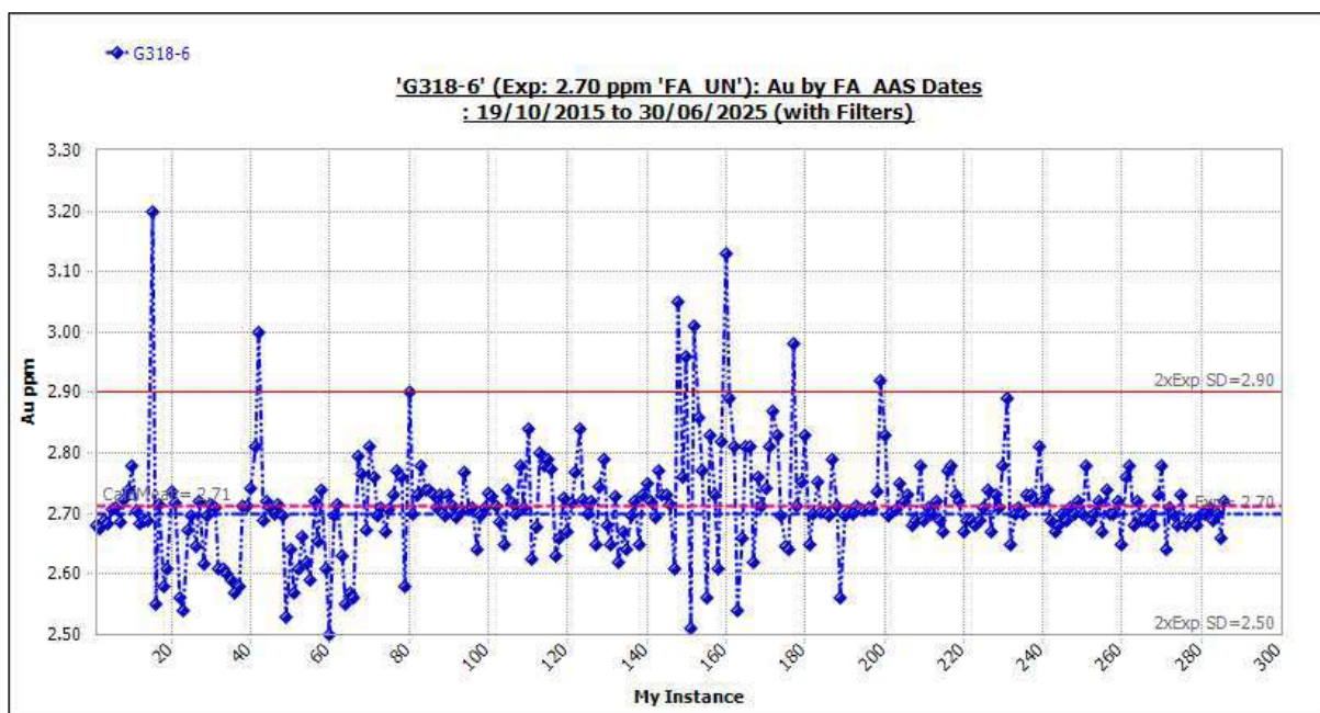
Figure 11-21 Standard G318-6: Outliers Included.
