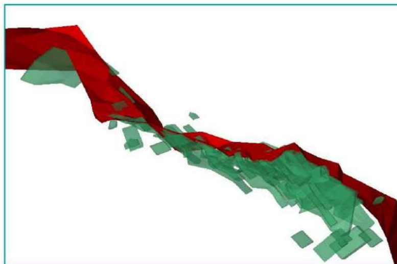
Figure 14-45 J2 wireframes (green) and dolerite (red) contact, looking northwest. Source: Westgold.
