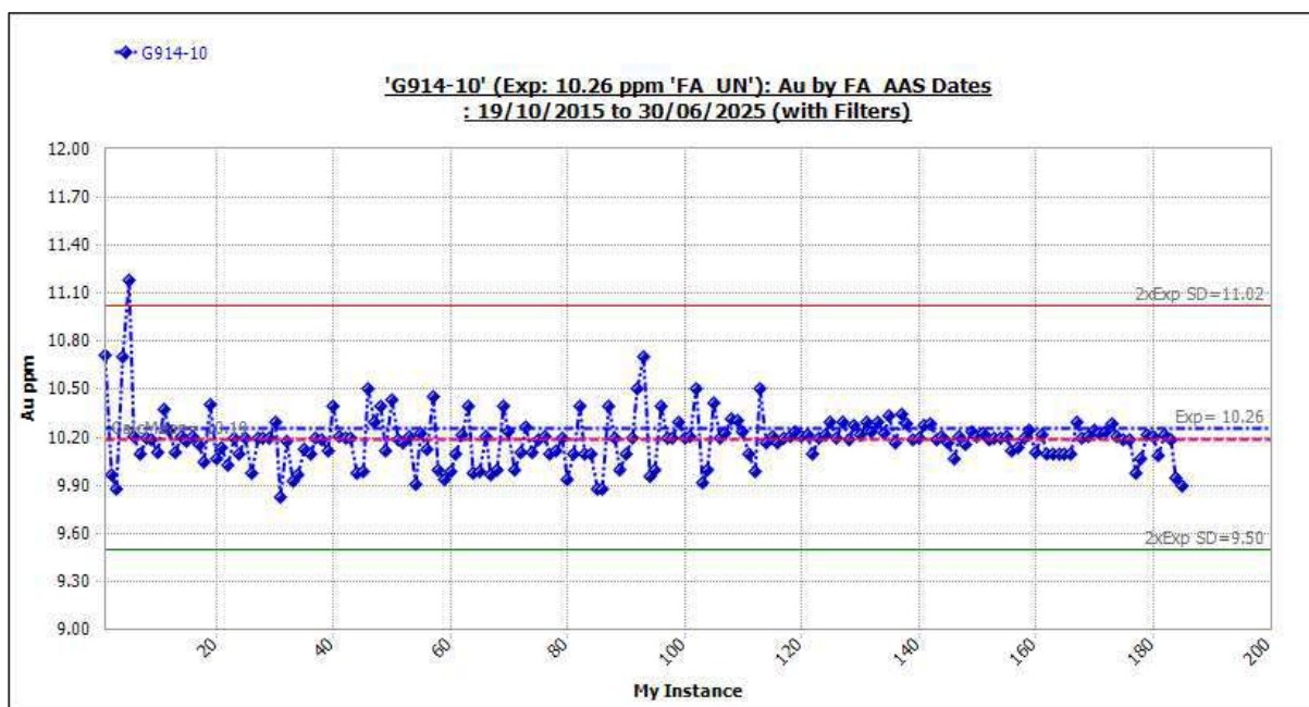
Figure 11-39 Standard G914-10: Outliers Included.
