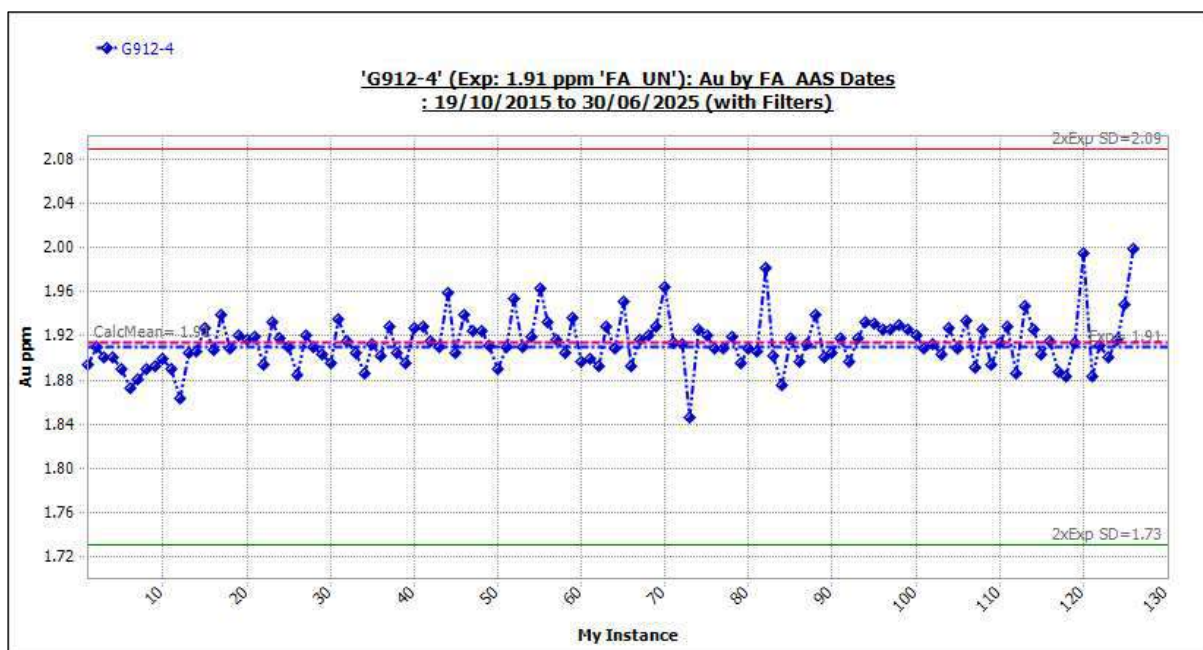
Figure 11-36 Standard G912-4: Outliers Included.
