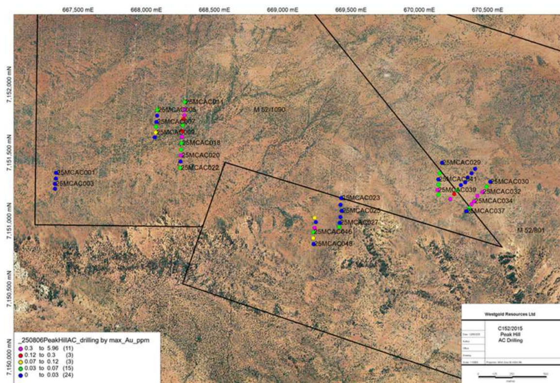
Figure 10-7 Murphy Creek drill program - Source: Westgold.
