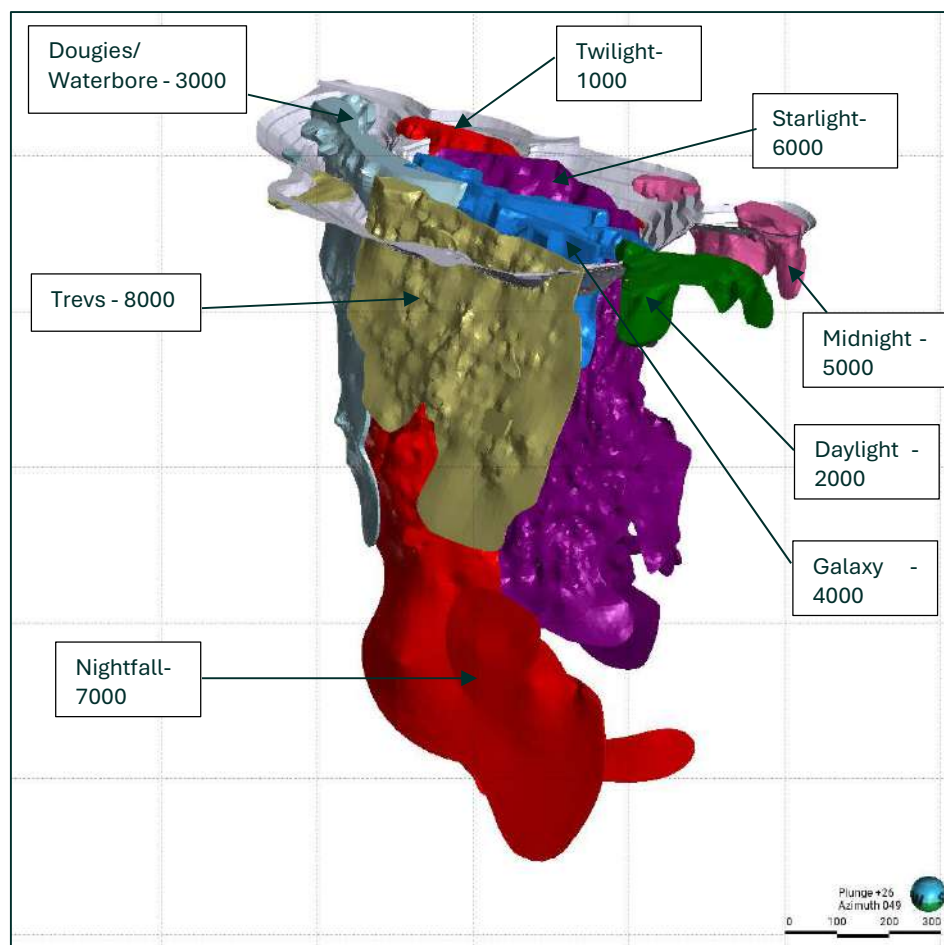
Figure 14-16 Oblique view of mineralisation domains - Source: Westgold.
