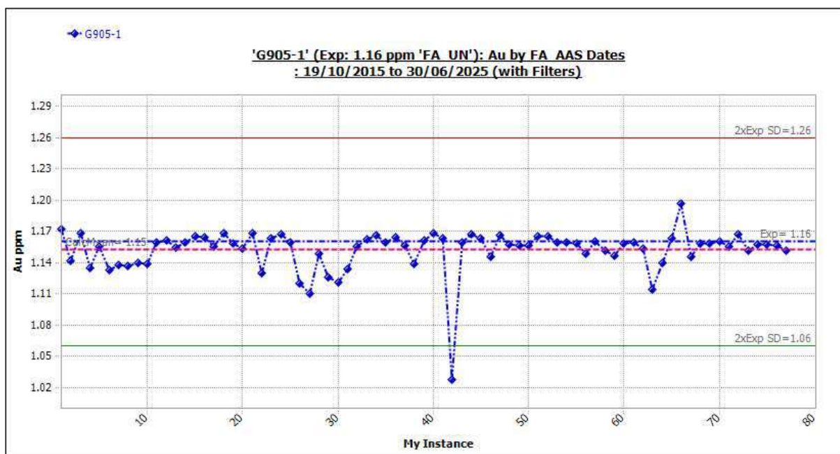
Figure 11-31 Standard G905-1: Outliers Included.
