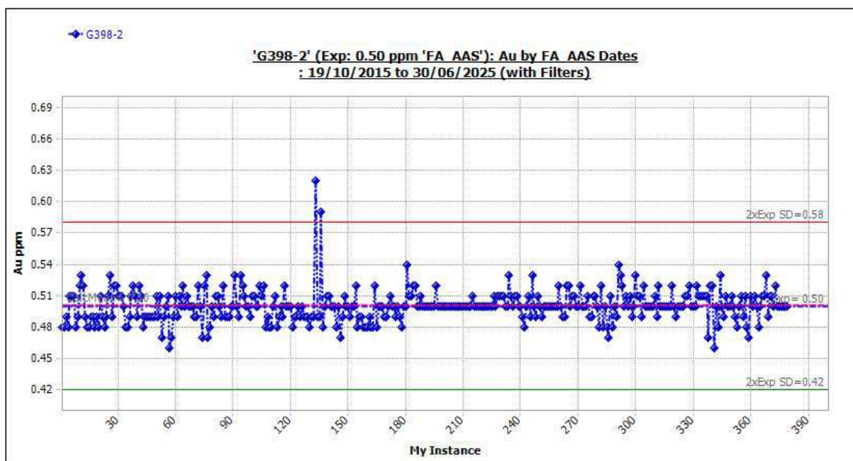
Figure 11-28 Standard G398-2: Outliers Included.
