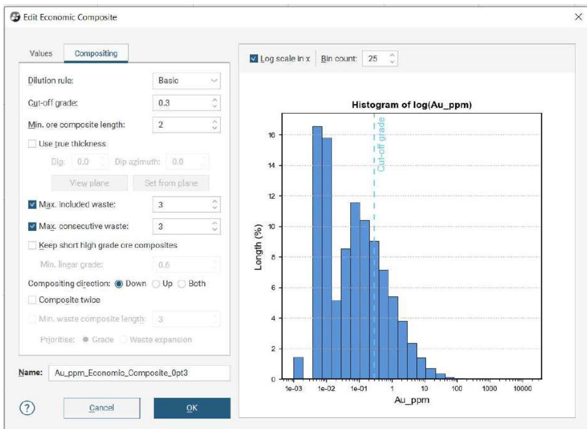
Figure 14-14 Leapfrog economic compositing parameters - Source: Westgold.
