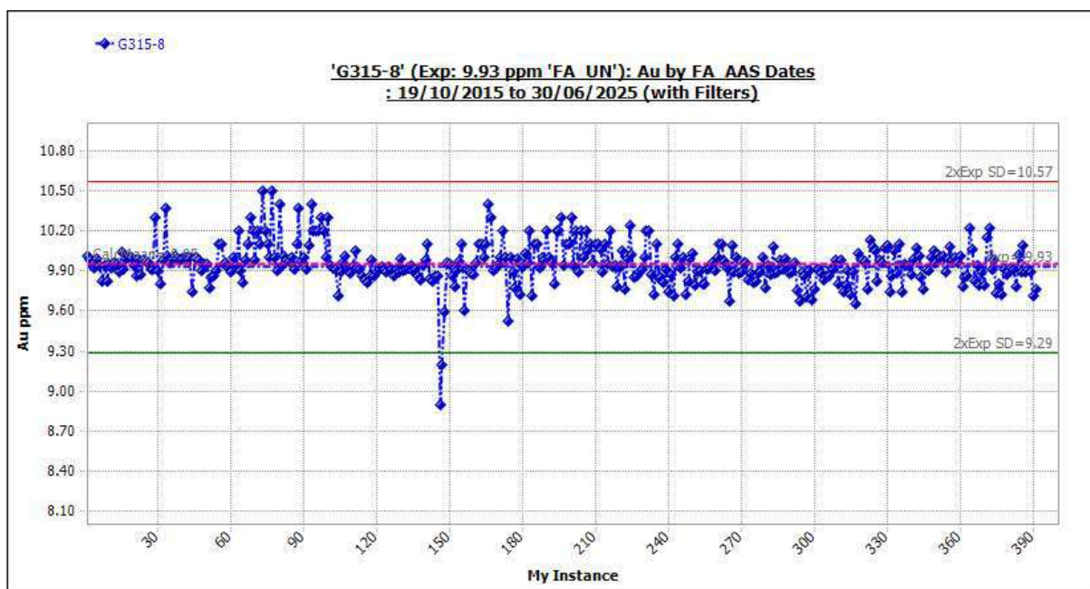
Figure 11-15 Standard G315-8: Outliers Included.
