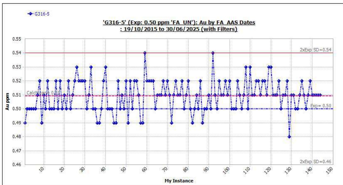
Figure 11-18 Standard G316-5: Outliers Included.
