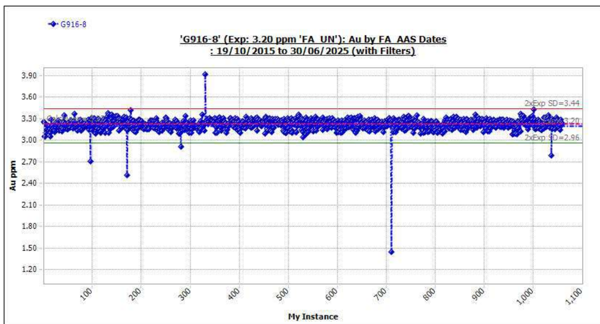
Figure 11-46 Standard G916-8: Outliers Included.
