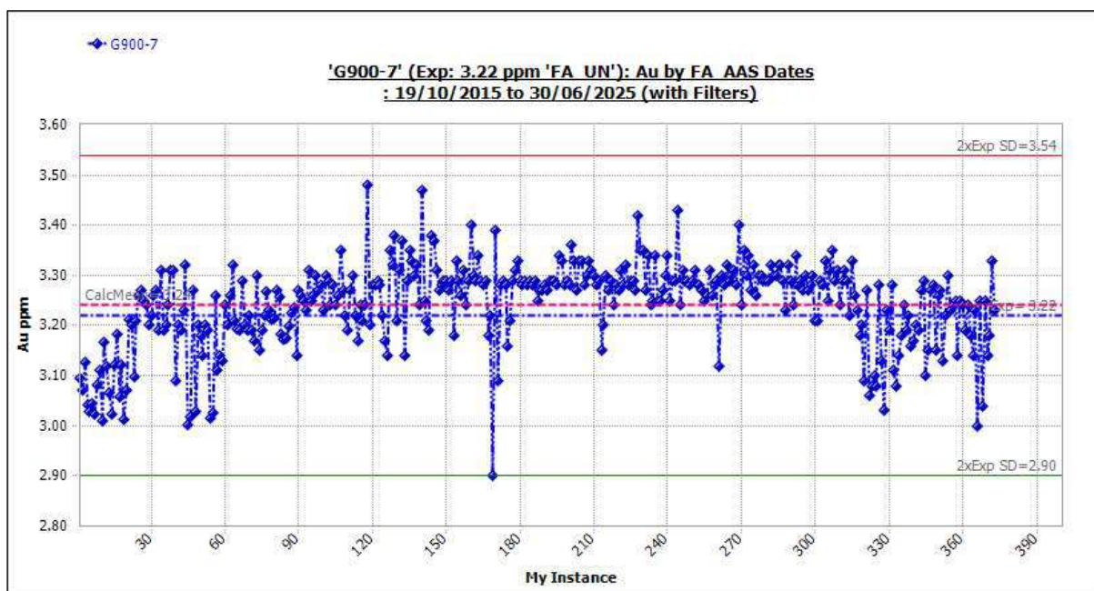
Figure 11-29 Standard G900-7: Outliers Included.
