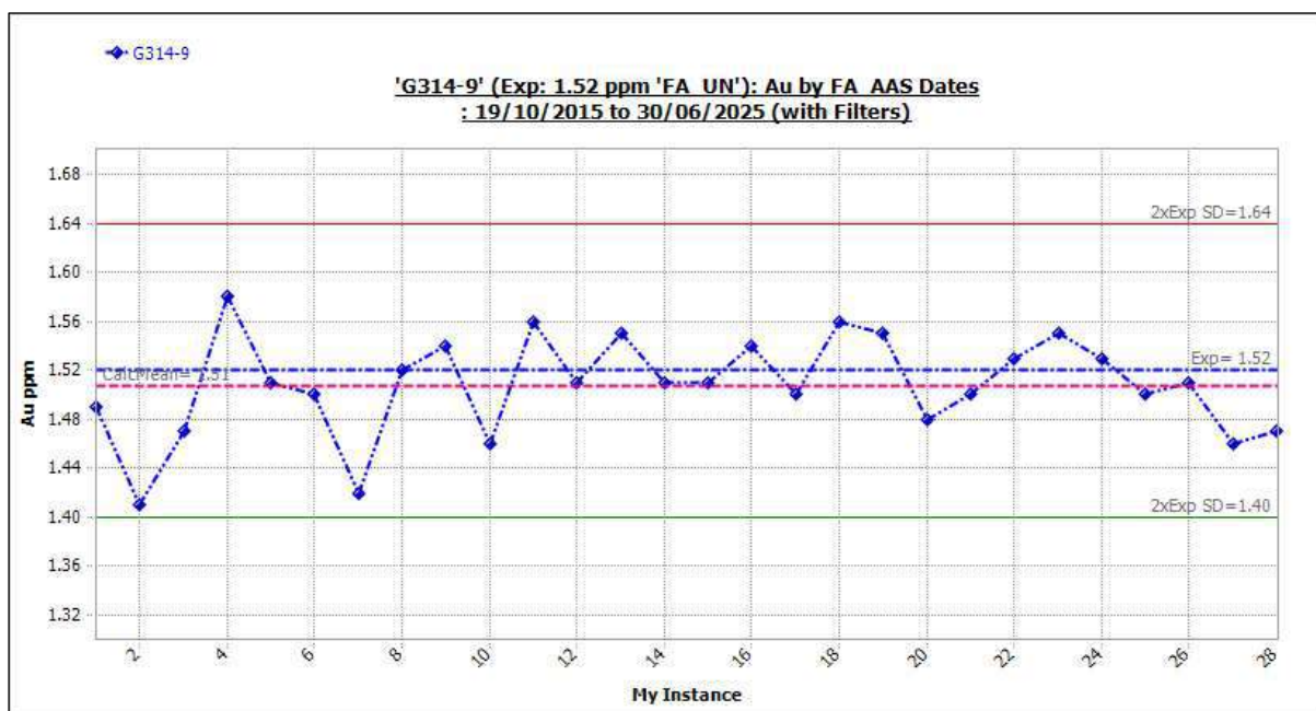
Figure 11-14 Standard G314-9: Outliers Included.
