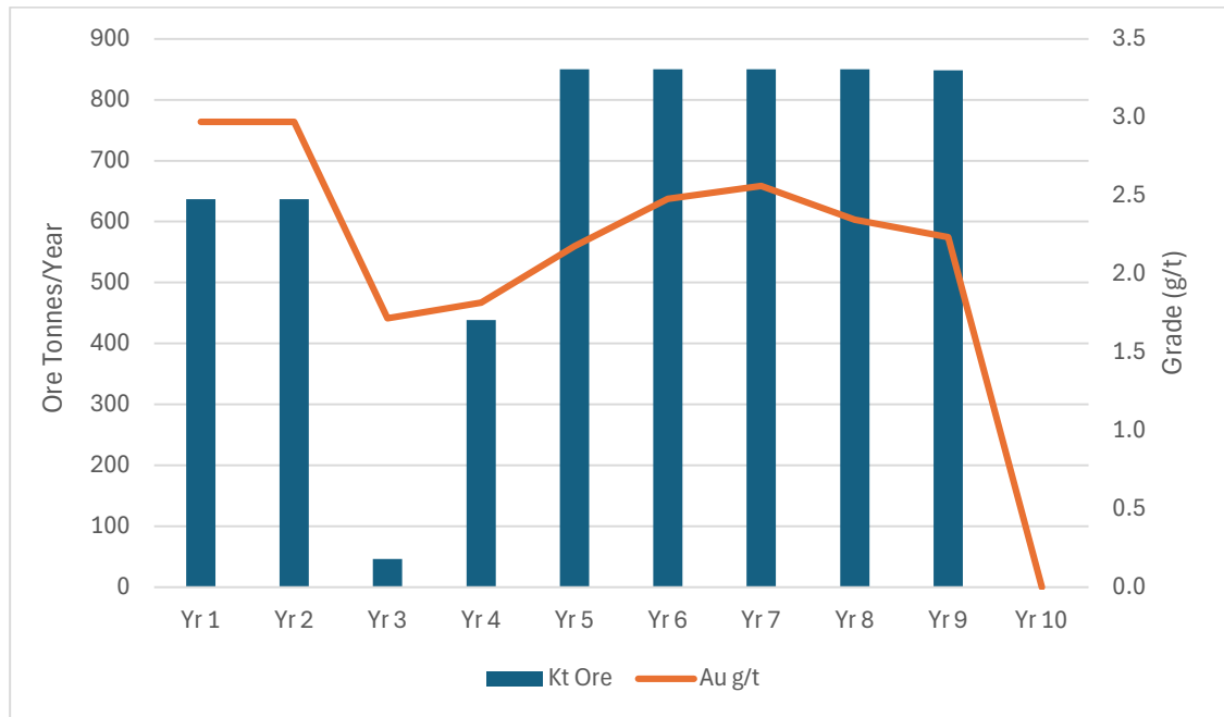
Figure 24-3 Key physical summary per year for underground – Source : Westgold.
