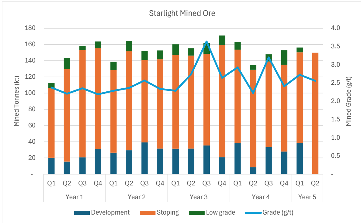
Figure 16-8 Starlight underground mining schedule. Source: Westgold.
