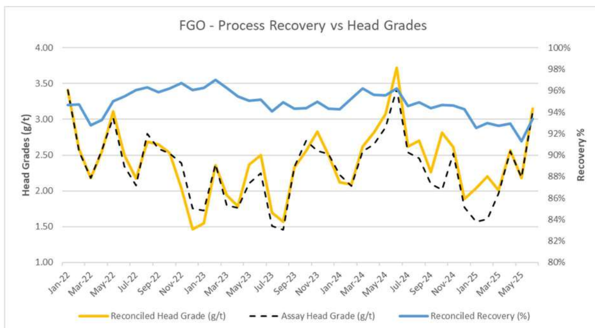
Figure 17-3 Fortnum process recoveries v. head grade - Source: Westgold.
