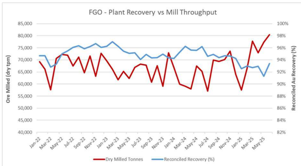
Figure 17-2 Fortnum process recoveries v. plant throughput. Source: Westgold.
