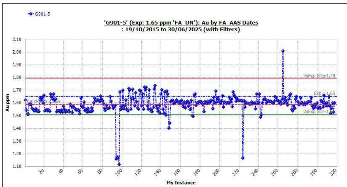
Figure 11-30 Standard G901-5: Outliers Included.
