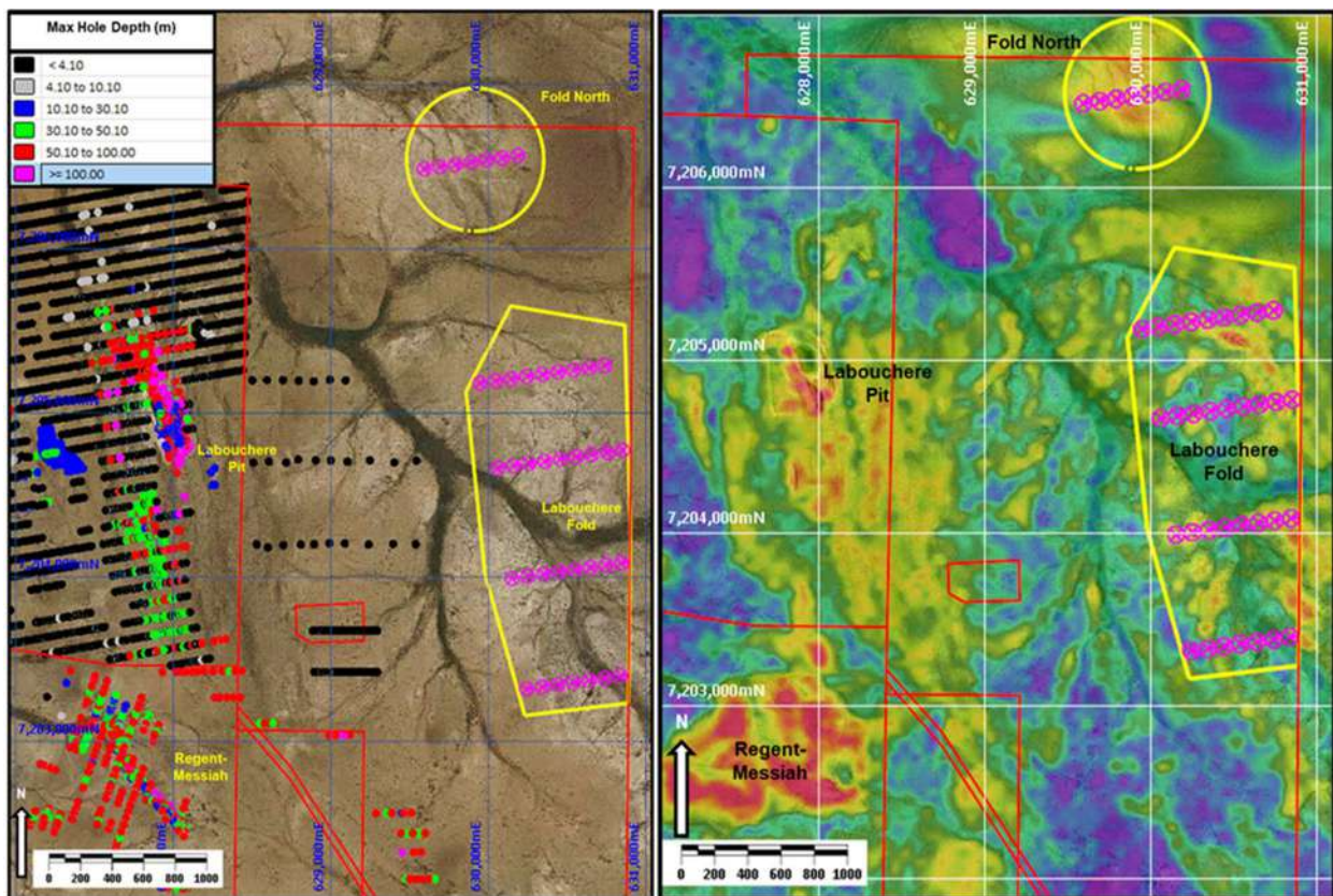
Figure 25-3 Historic and planned drillhole locations at Labouchere Fold. Displaying limited and shallow drilling. (Right) Radiometric potassium (K) data over the Labouchere area - Source: Westgold, 2025.
