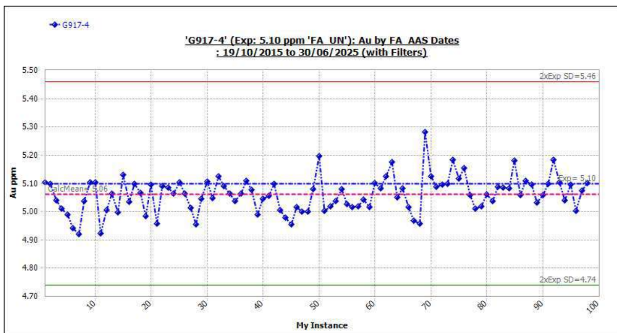
Figure 11-48 Standard G917-4: Outliers Included.
