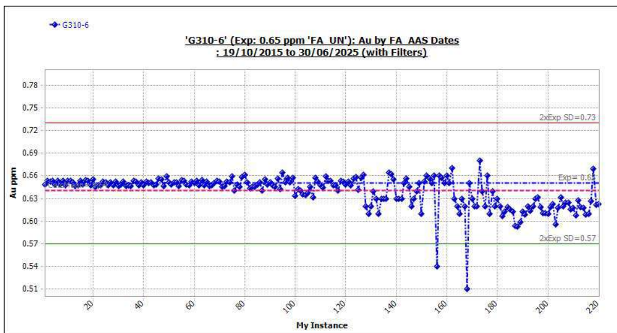
Figure 11-5 Standard G310-6: Outliers Included.
