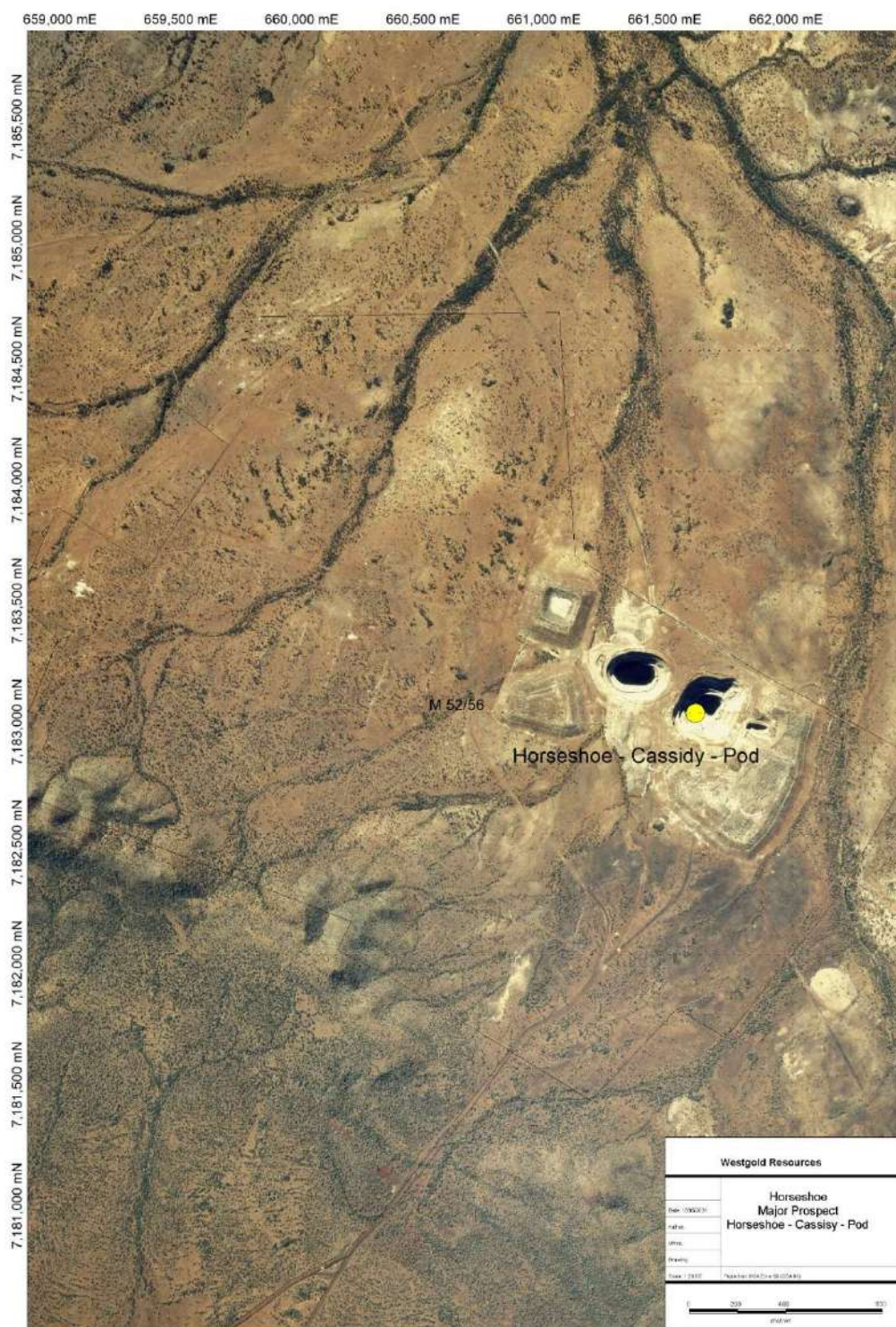
Figure 14-29 Horseshoe – Cassidy - Pod deposit location map. Source: Westgold.
