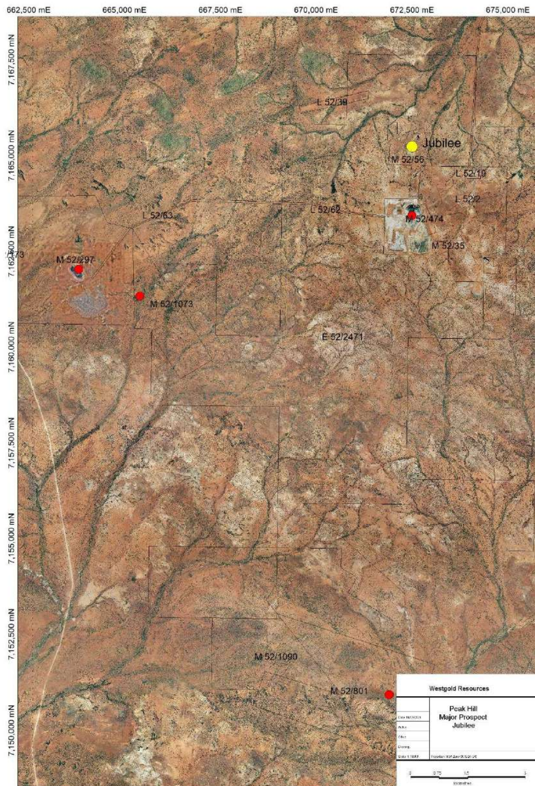
Figure 14-44 Jubilee deposit location map. Source: Westgold.
