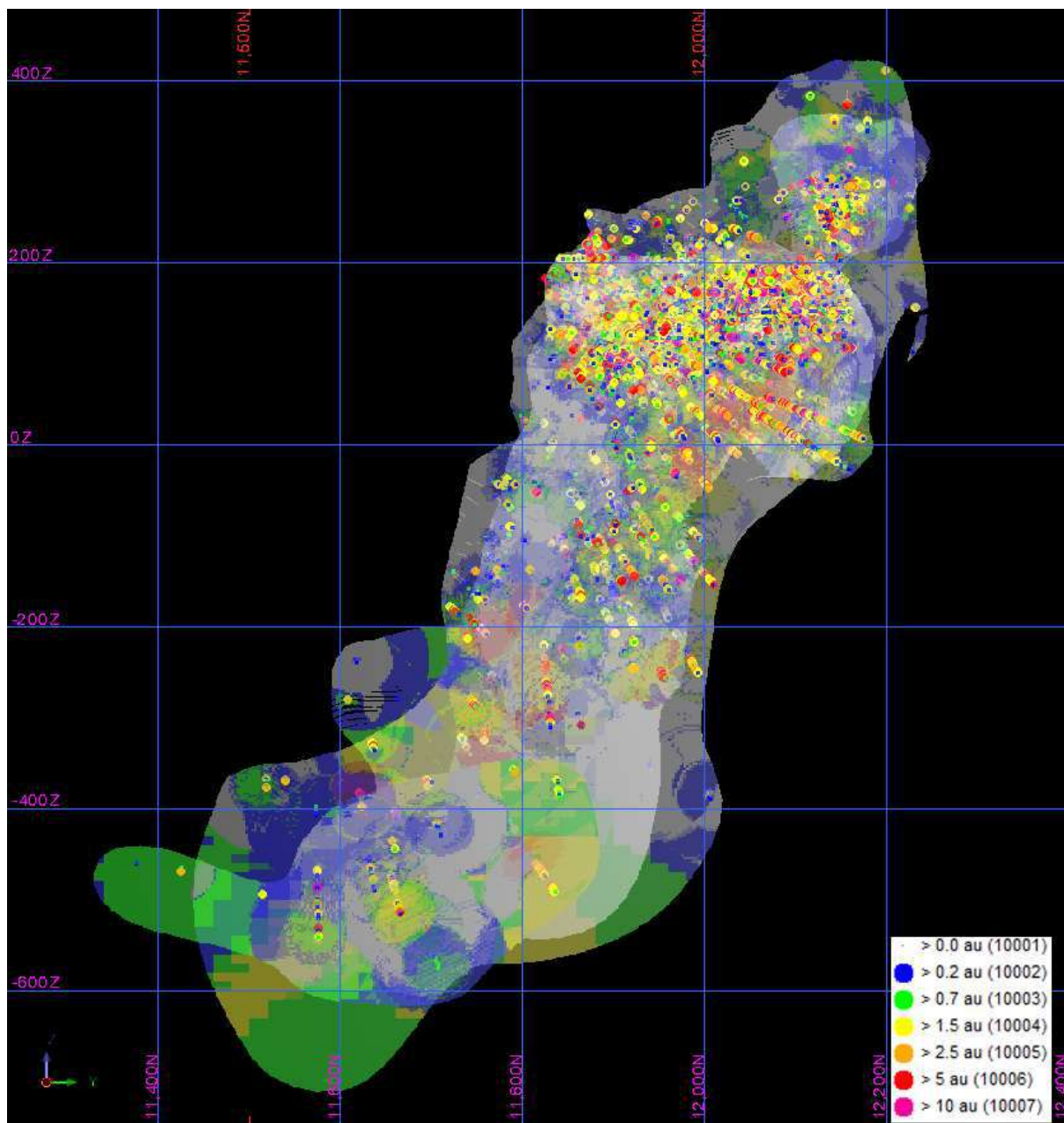
Figure 14-21 Domain 7000 - Nightfall blocks versus composite data (coloured by au_final ) – Note the large number of LG blocks at depth informed by relatively few samples - Source: Westgold.
