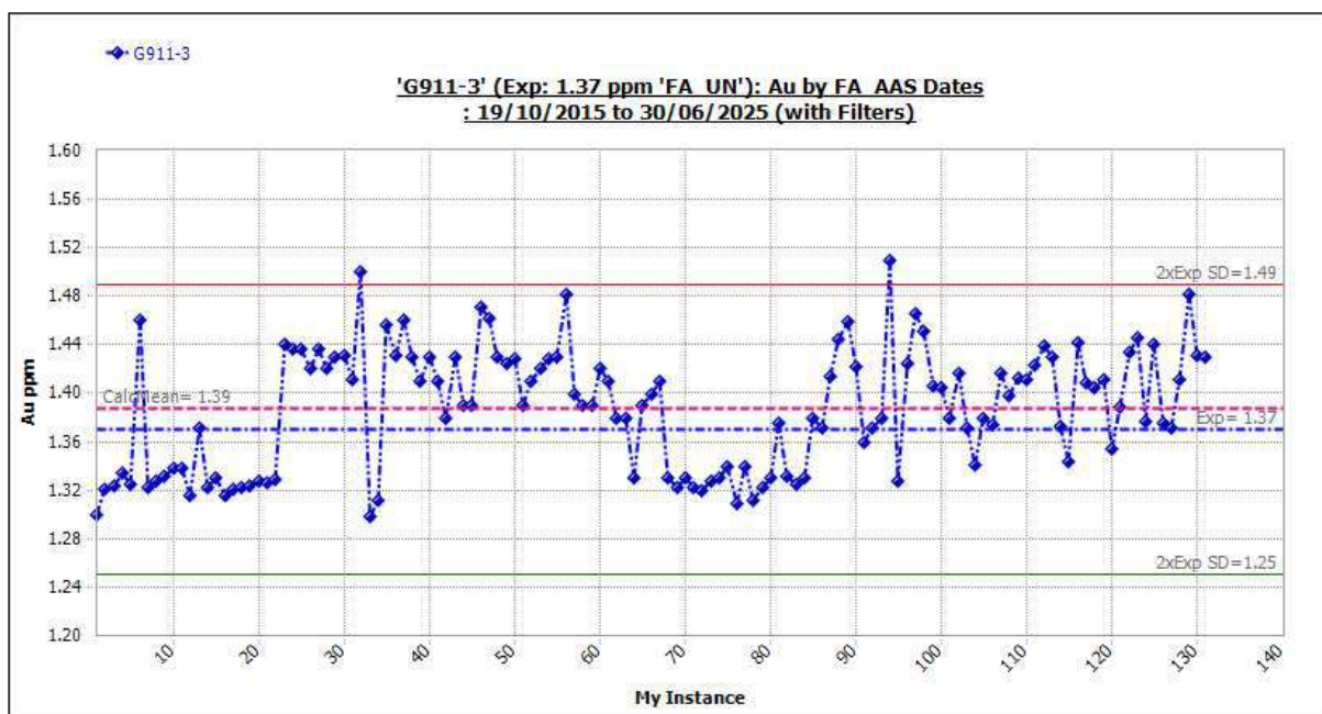
Figure 11-34 Standard G911-3: Outliers Included.
