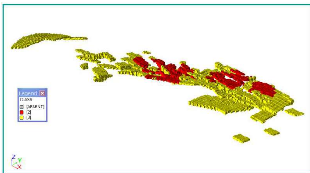
Figure 14-48 J2 block model classification (red = Indicated, yellow = Inferred). Source: Westgold.
