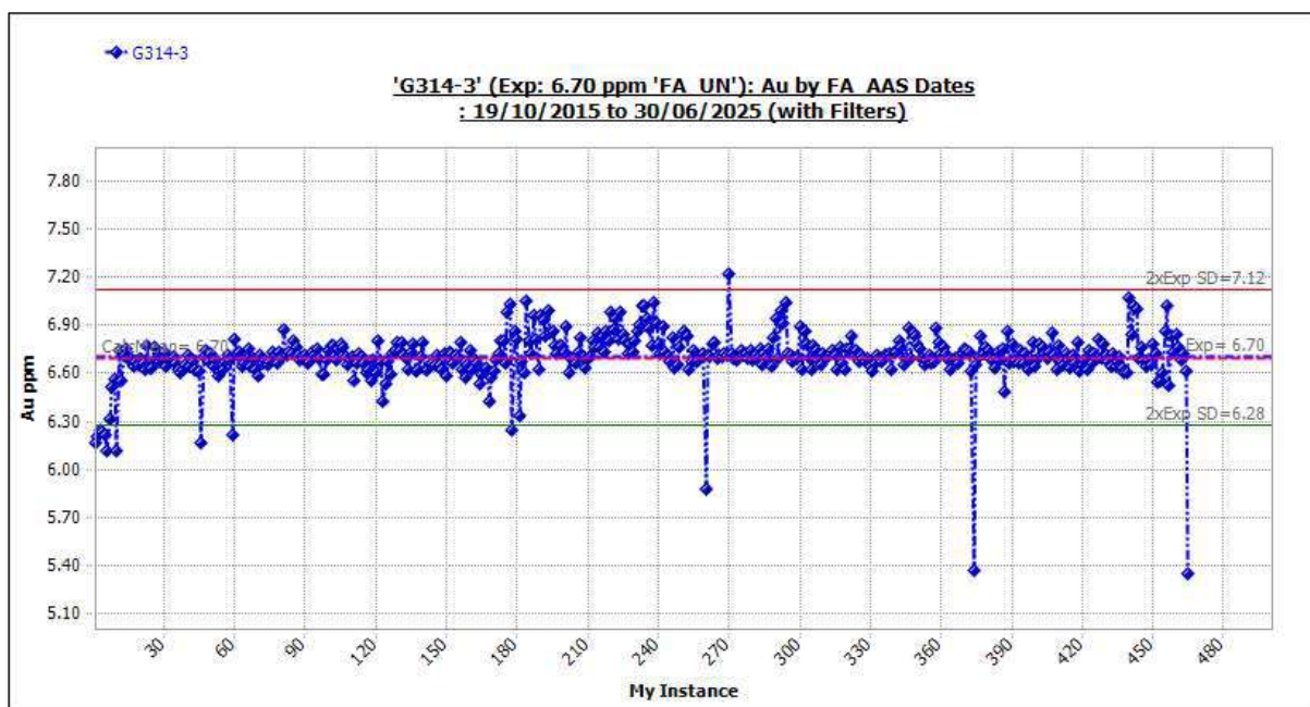
Figure 11-12 Standard G314-3: Outliers Included.
