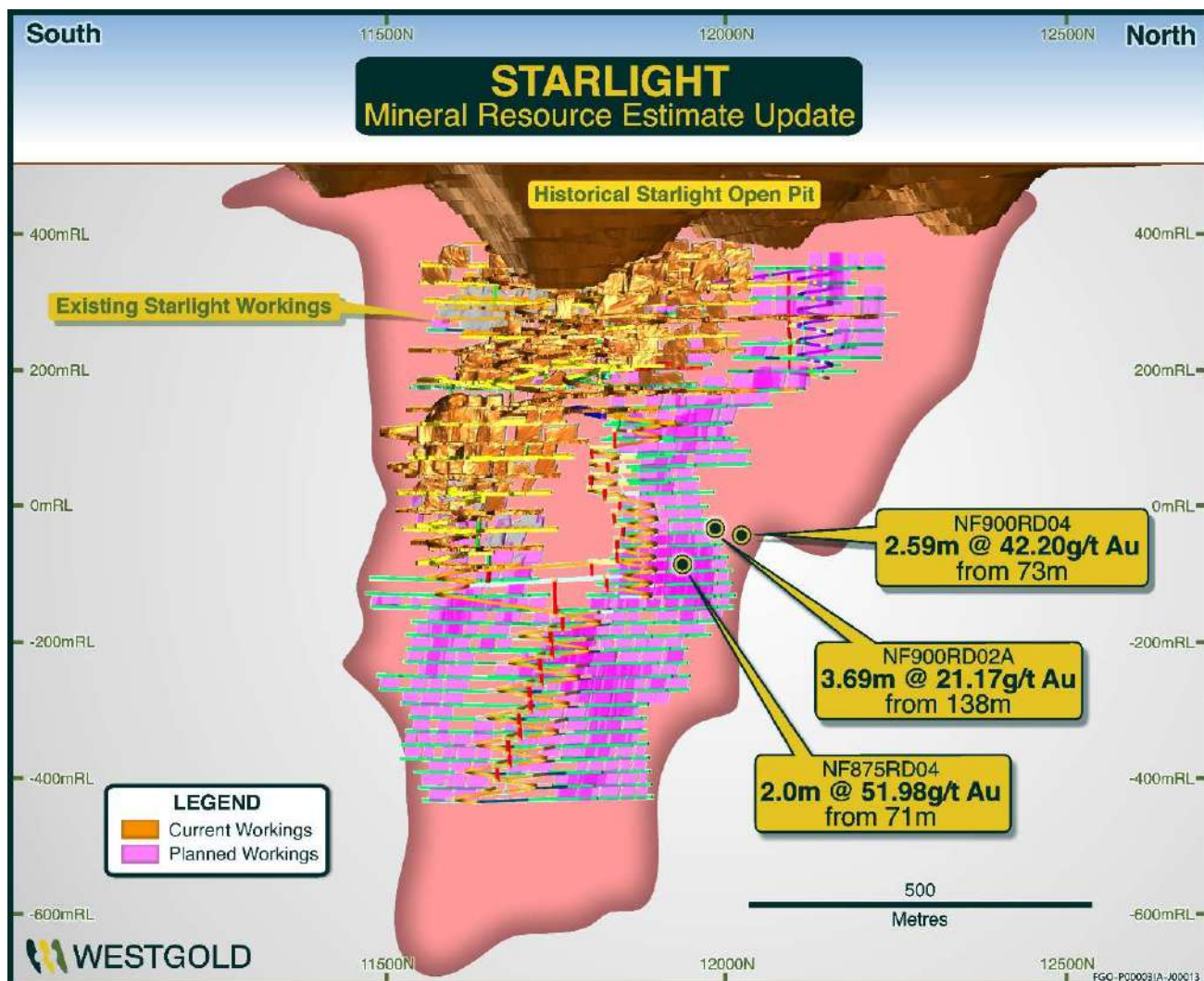
Figure 10-2 FY2025 Selected Starlight Significant Intersections - Source: Westgold.
