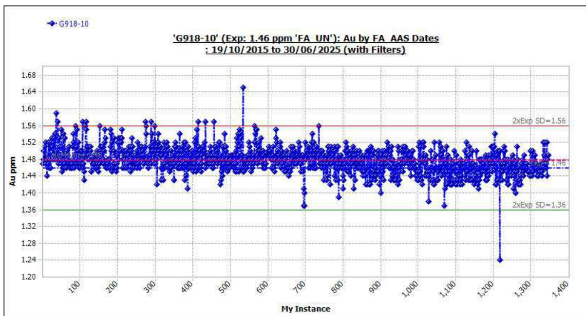
Figure 11-50 Standard G918-10: Outliers Included.
