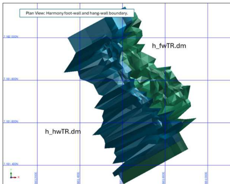
Figure 14-42 Harmony mineralisation wireframes plan view. Source: Westgold.
