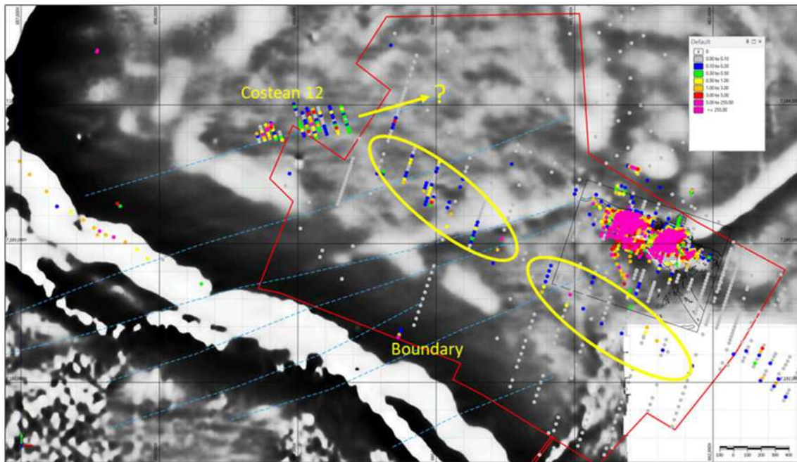
Figure 25-4 Horseshoe North M52/338 lease displaying magnetics, max downhole Au and interpreted northeast-trending structures (blue) - Source: Westgold, 2025.
