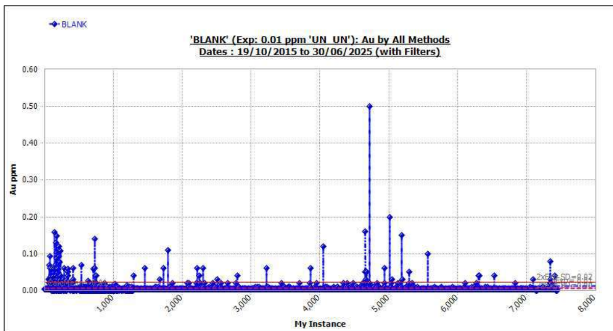
Figure 11-3 Standard BLANK: Outliers Included.
