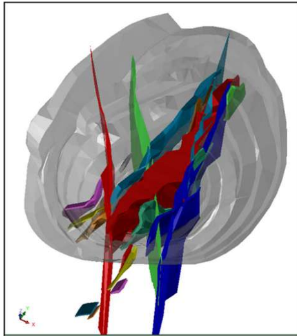
Figure 14-7 Nathan's isometric view of mineralisation wireframes, 1992 pit survey, 130° fault (red). Source: Westgold.
