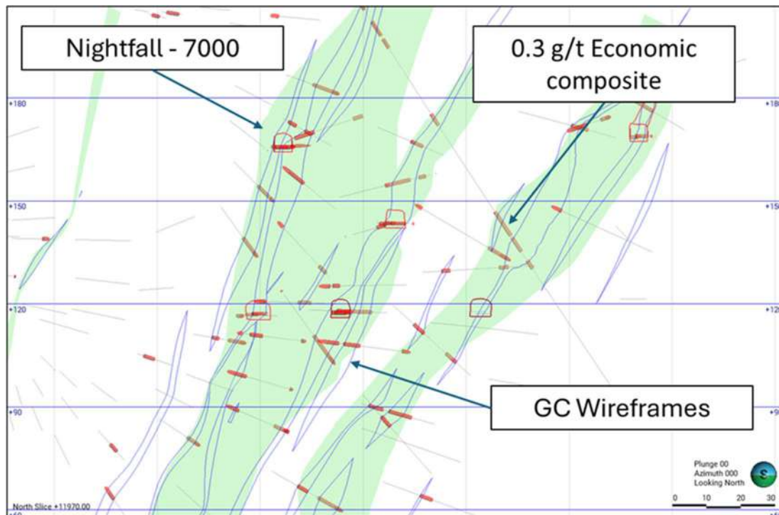
Figure 14-15 Cross section of the Nightfall wireframe (green) showing the internal GC wireframes (blue) - Source: Westgold.
