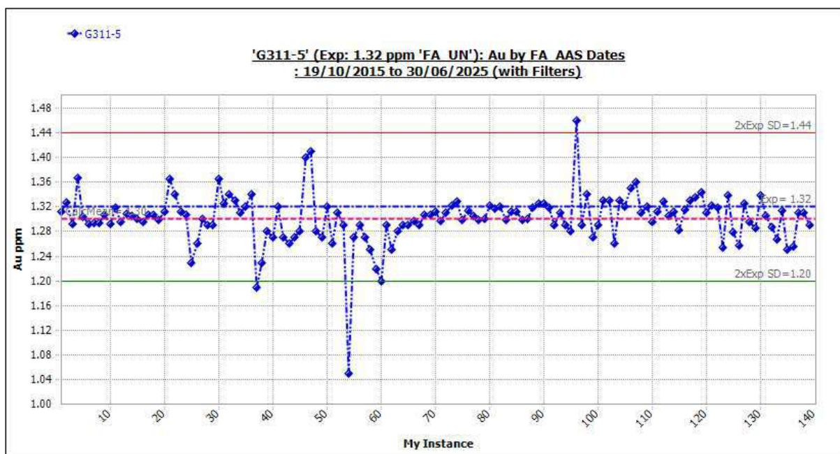
Figure 11-6 Standard G311-5: Outliers Included.
