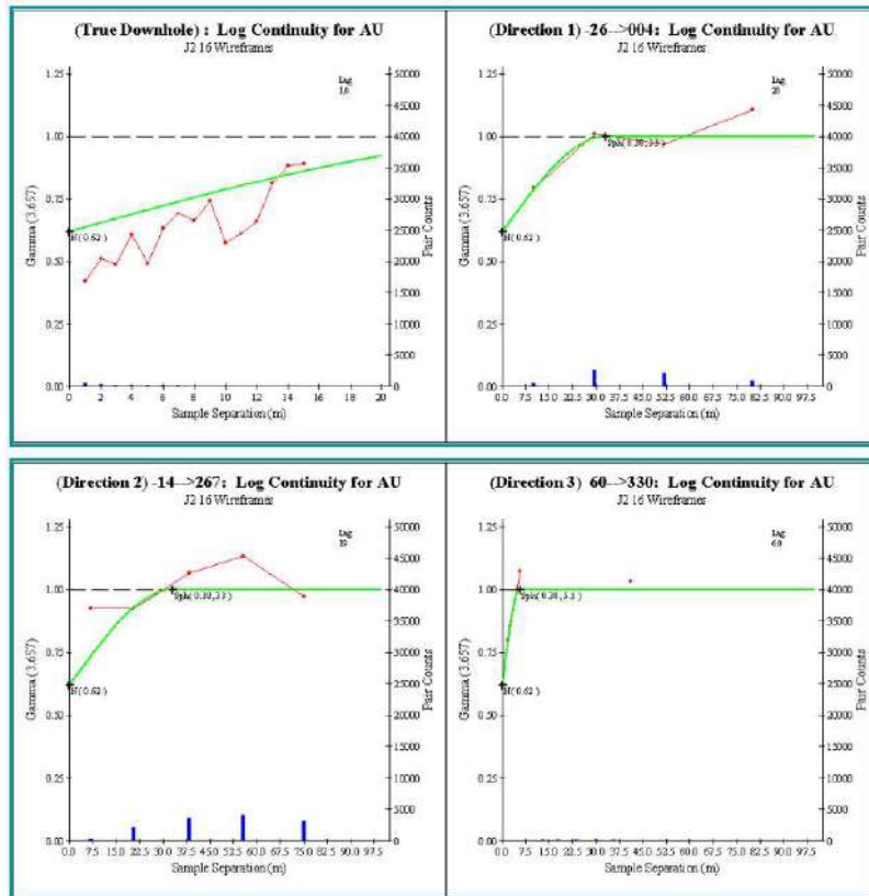
Figure 14-46 J2 Variograms. Source: Westgold.
