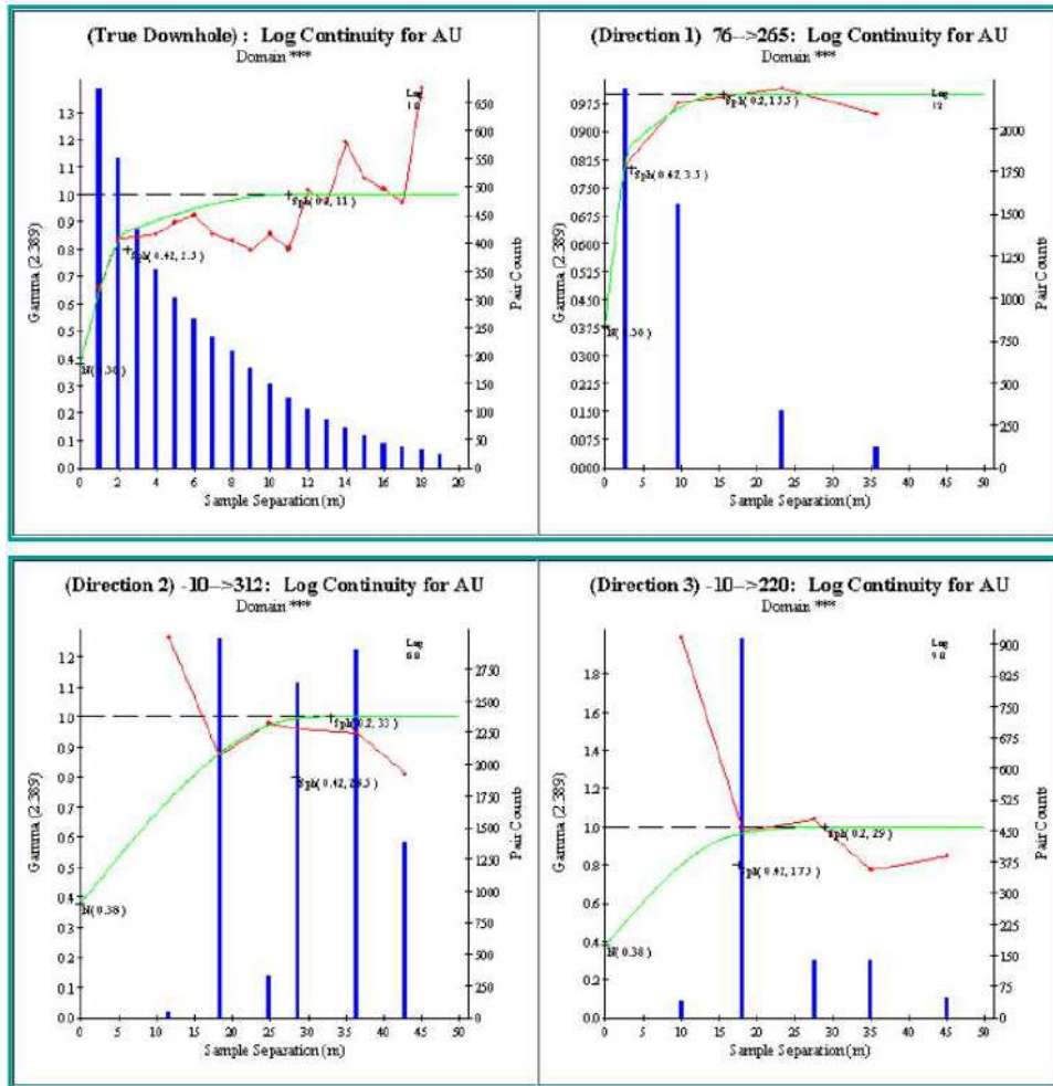
Figure 14-47 J3 Variograms. Source: Westgold.
