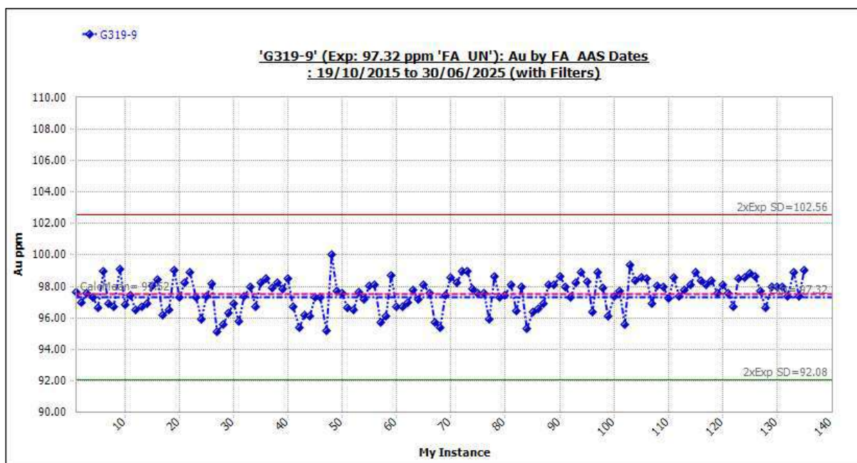
Figure 11-25 Standard G319-9: Outliers Included.
