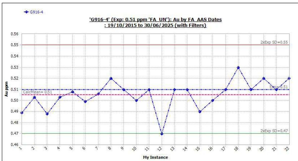
Figure 11-45 Standard G916-4: Outliers Included.
