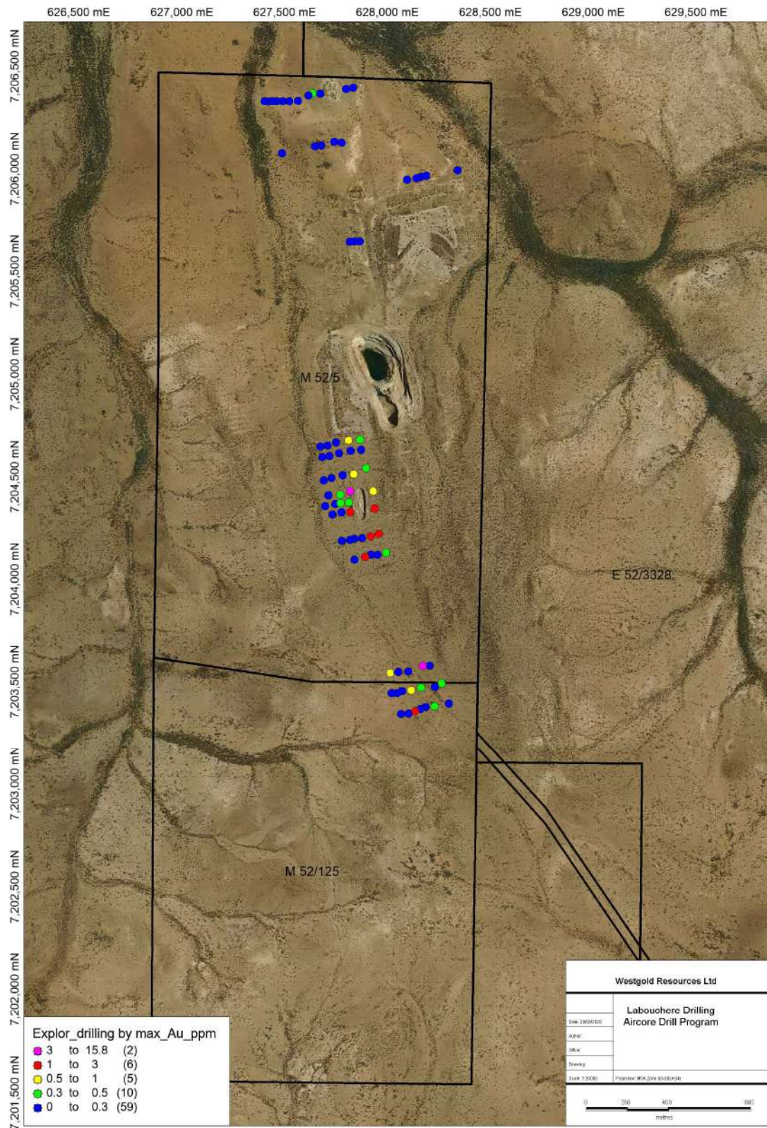
Figure 10-3 Drilling north of Labouchere pit testing for buried deeper mineralisation and drilling around the Central Valley pit on M52/125 and the Rebel prospect on M52/5 and into M52/125 - Source: Westgold.
