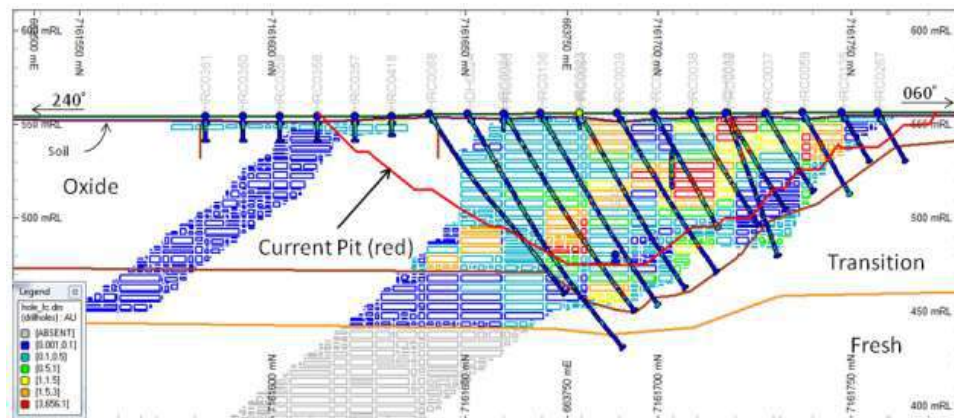
Figure 14-43 Visual comparison of gold grades at Harmony between drillholes and block model. Source: Westgold.
