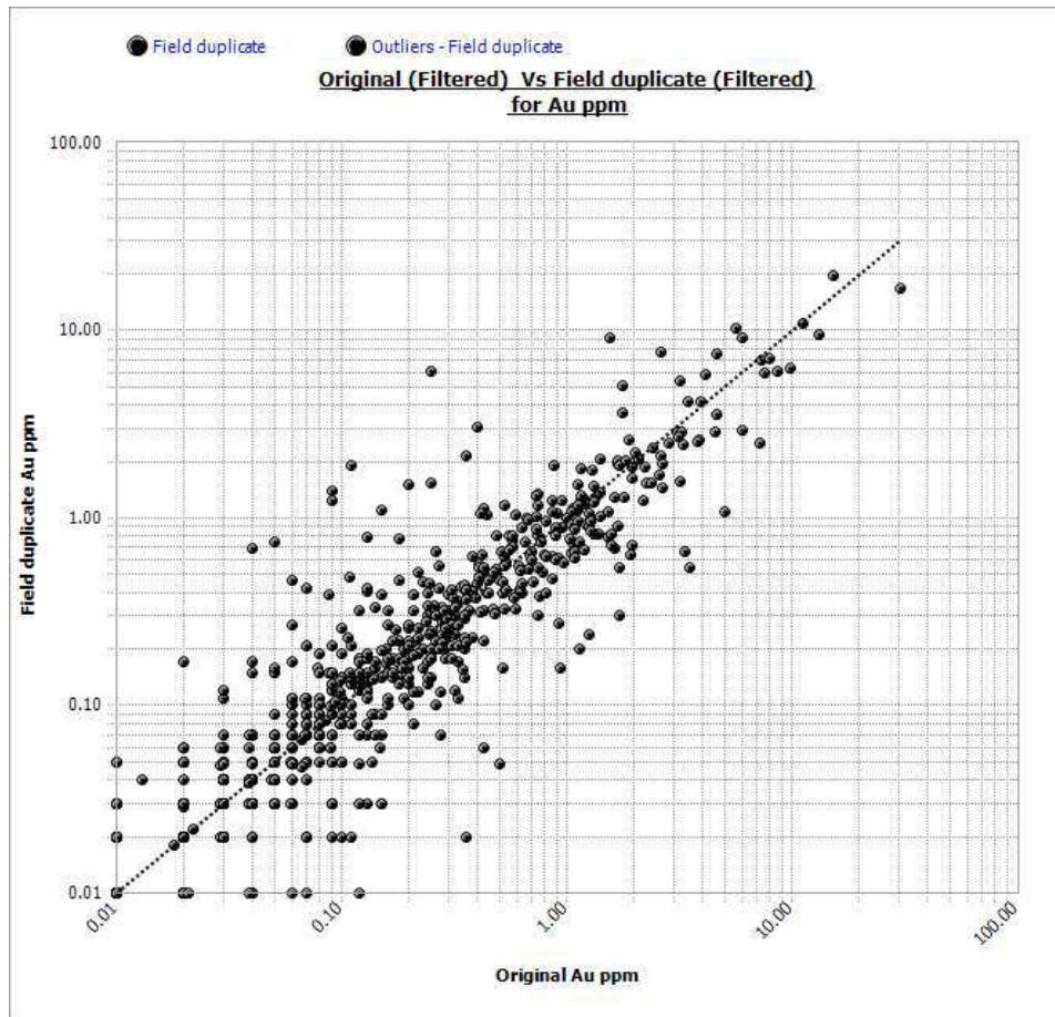
Figure 11-57 Q-Q Plot - drillhole (Repeat Code) : original v. field duplicate for Au ppm.
