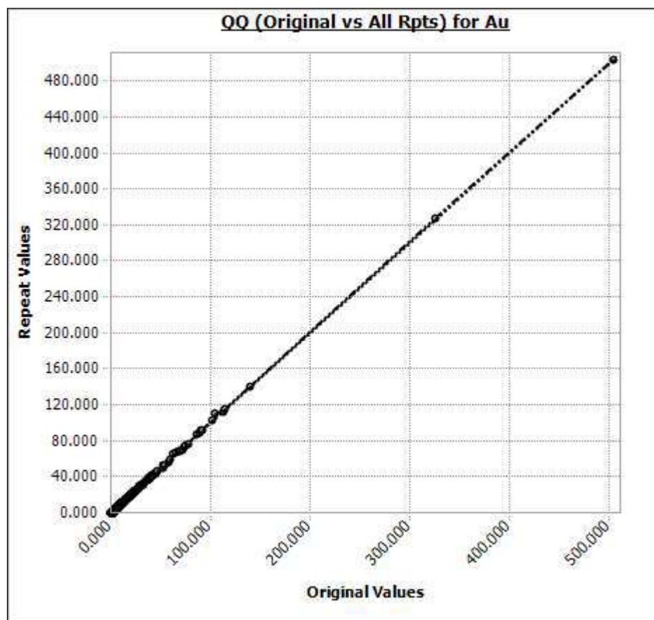
Figure 11-54 Q-Q Plot - Drillhole (Repeat Code) : Original v. All Rpts for Au ppm.
