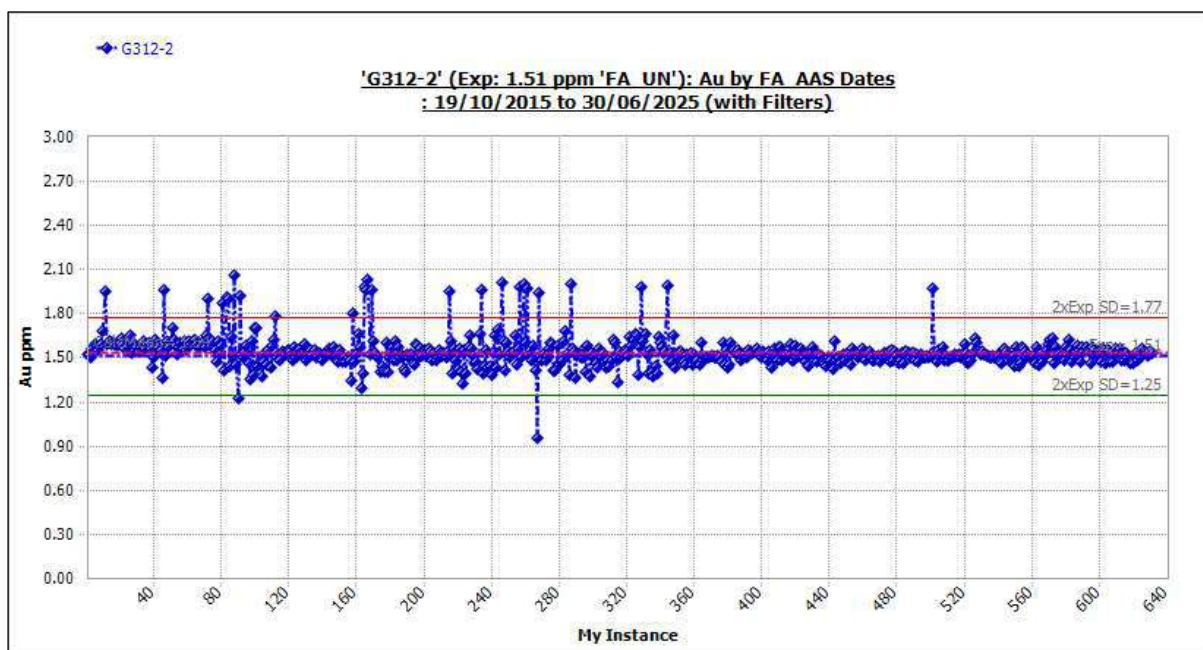
Figure 11-8 Standard G312-2: Outliers Included.
