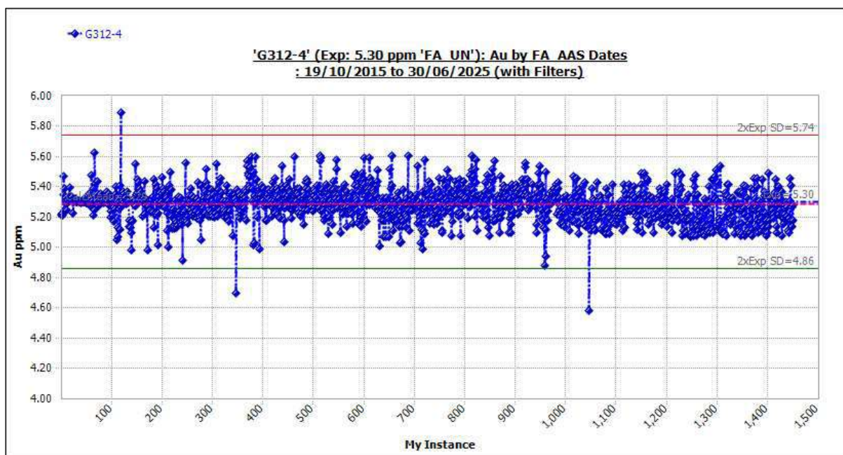
Figure 11-9 Standard G312-4: Outliers Included.
