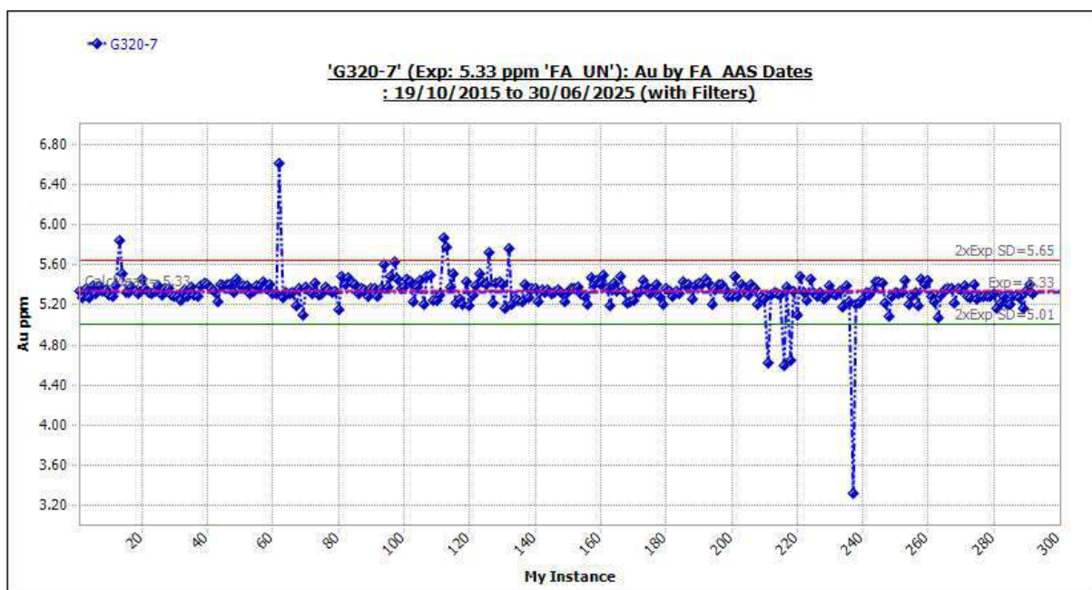
Figure 11-26 Standard G320-7: Outliers Included.
