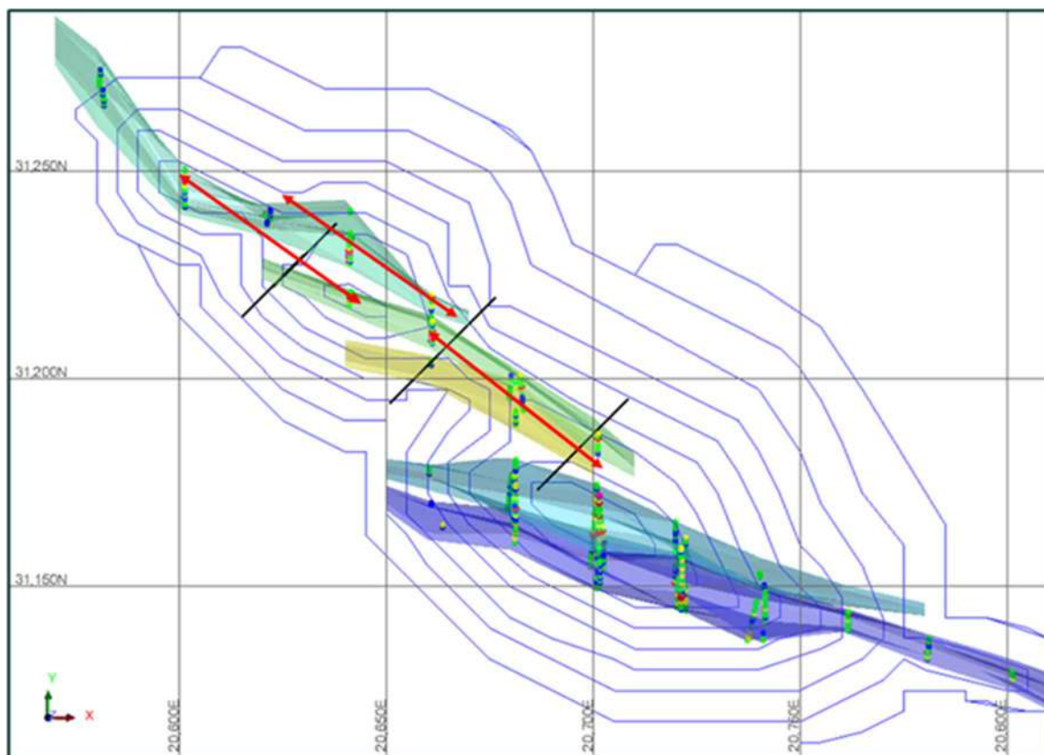
Figure 14-11 Plan view of the Messiah deposit showing the existing drill holes (Au grade distributions), planned holes (thick black lines). Source: Westgold.
