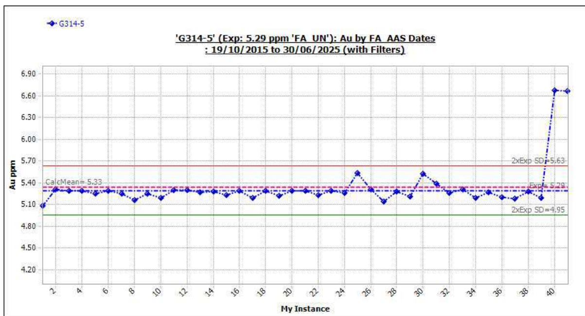
Figure 11-13 Standard G314-5: Outliers Included.
