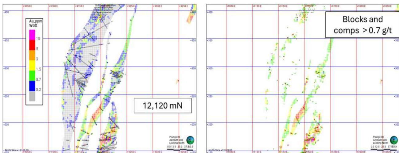
Figure 14-23 Cross section view at 12,120mN; Au ppm block grades versus gold assays – all samples (left) and above a 0.7 g/t (right) - Source: Westgold.
