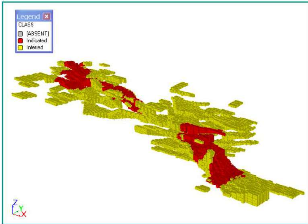
Figure 14-49 J3 block model classification (red = Indicated, yellow = Inferred). Source: Westgold.
