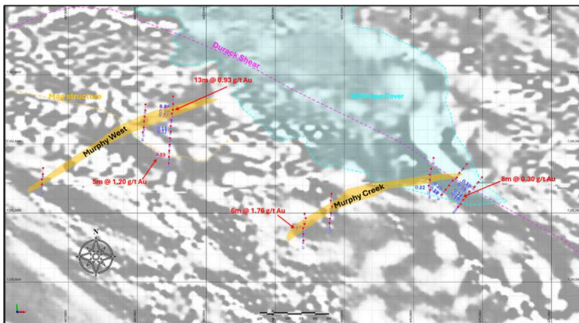
Figure 10-8 Plan view map of Murphy Creek target area. Drill holes (red) along with interpreted mineralising trends and selected significant intercepts from E2024-PKH-003 - Source: Westgold.
