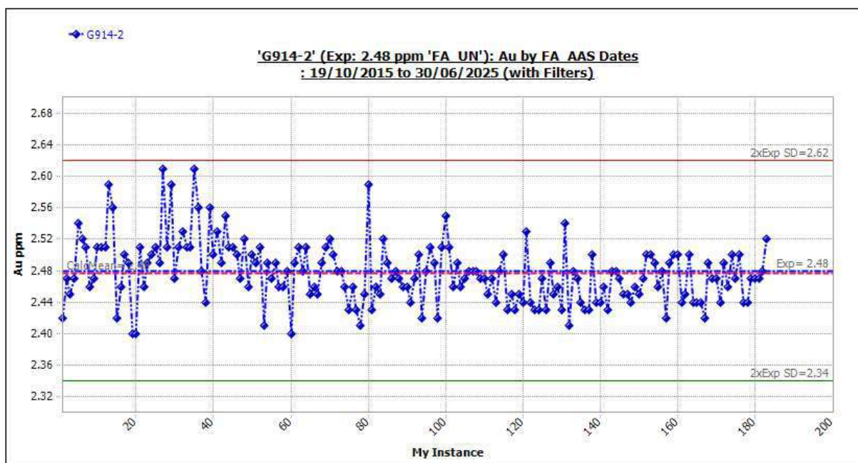
Figure 11-40 Standard G914-2: Outliers Included.
