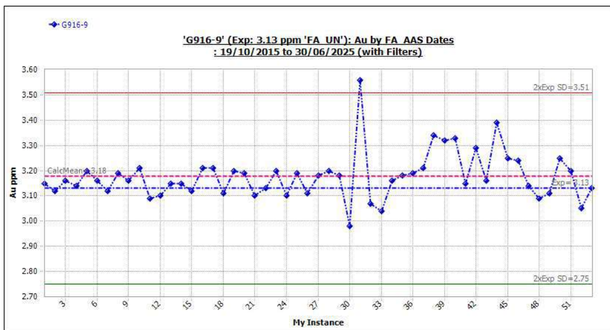
Figure 11-47 Standard G916-9: Outliers Included.
