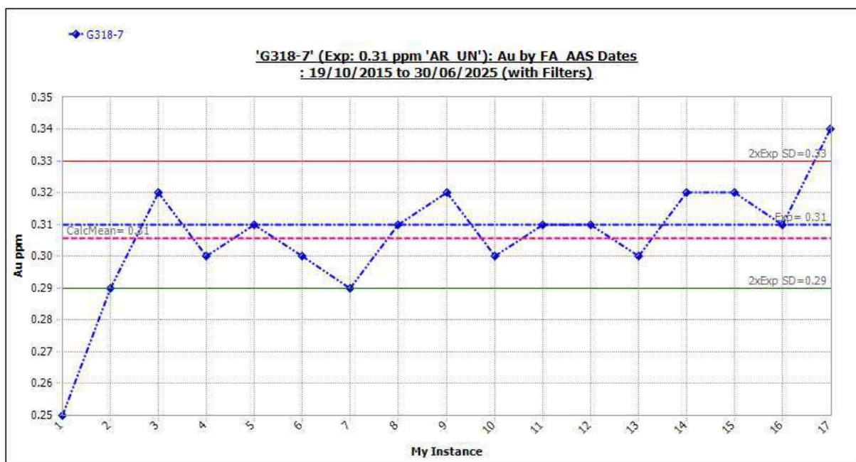
Figure 11-22 Standard G318-7: Outliers Included.
