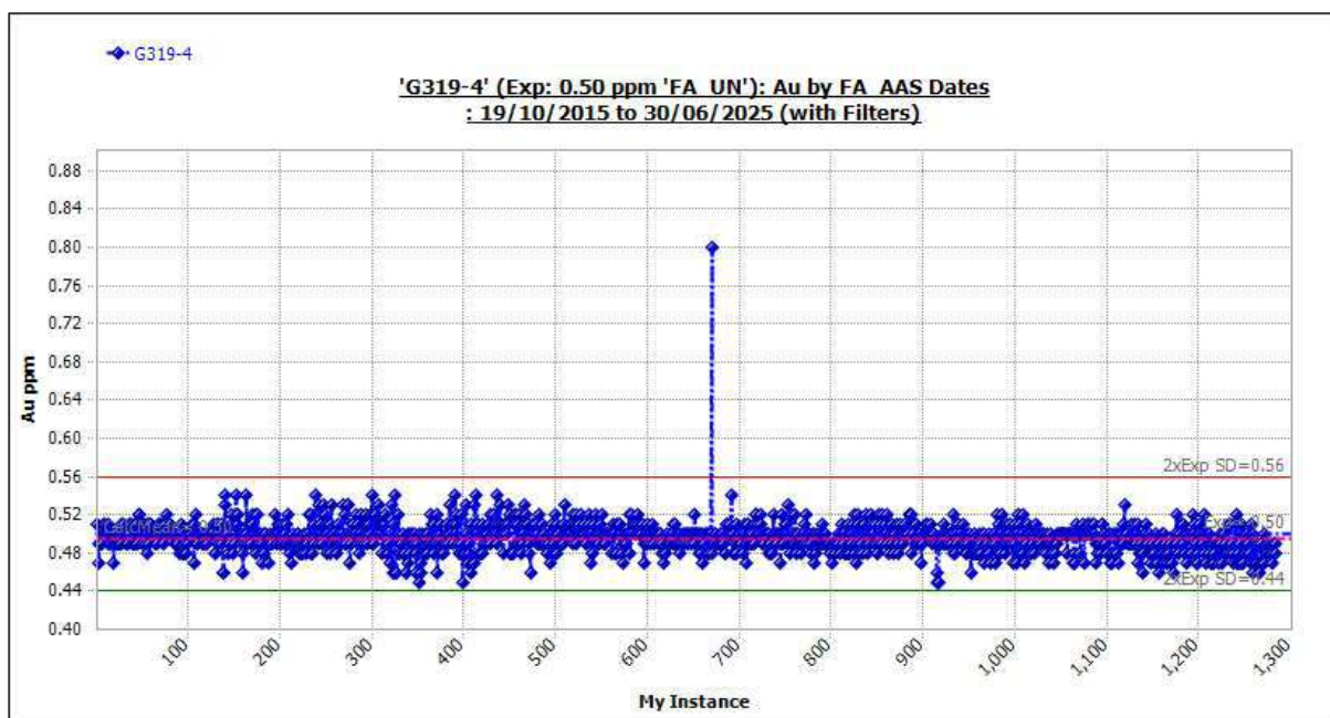
Figure 11-24 Standard G319-4: Outliers Included.
