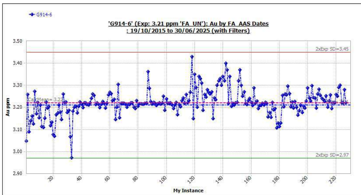
Figure 11-41 Standard G914-6: Outliers Included.
