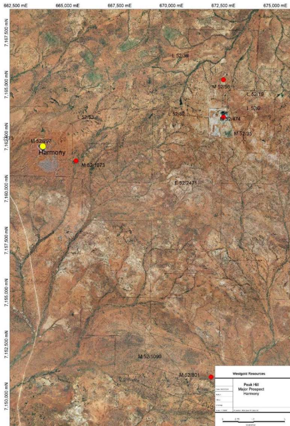
Figure 14-41 Harmony deposit location map. Source: Westgold.
