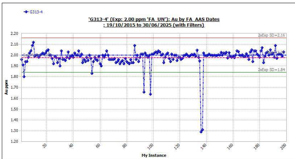
Figure 11-11 Standard G313-4: Outliers Included.
