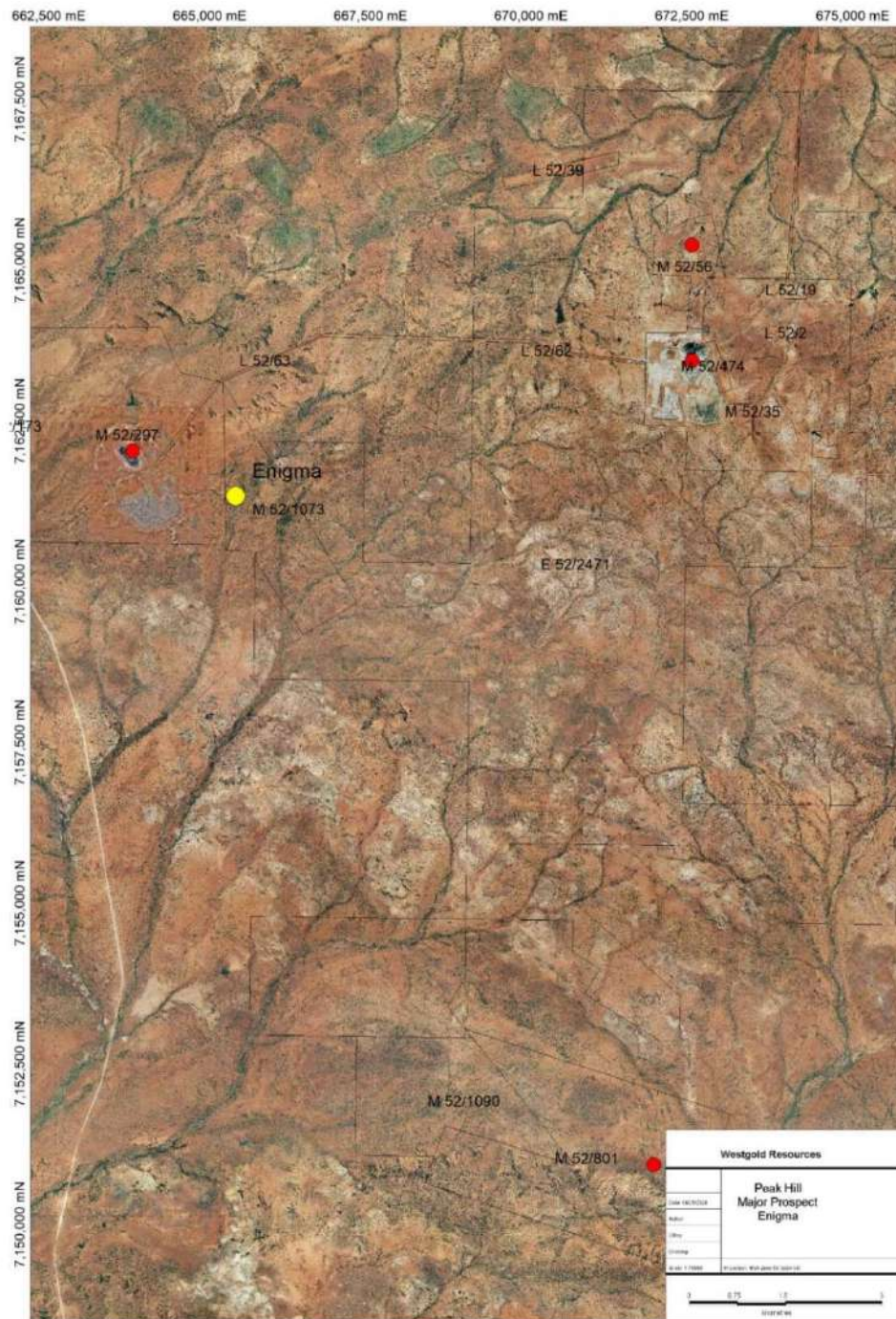
Figure 14-35 Enigma deposit location map. Source: Westgold.
