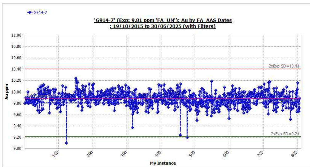
Figure 11-42 Standard G914-7: Outliers Included.
