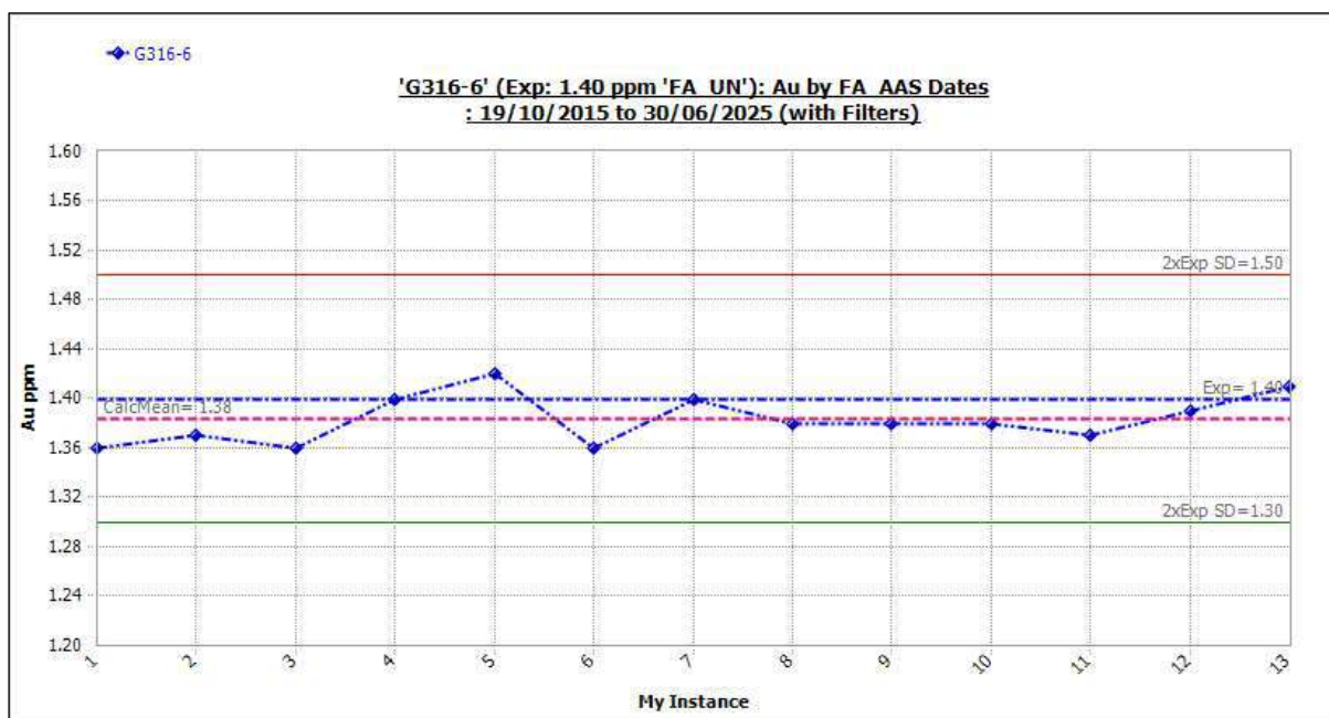
Figure 11-19 Standard G316-6: Outliers Included.
