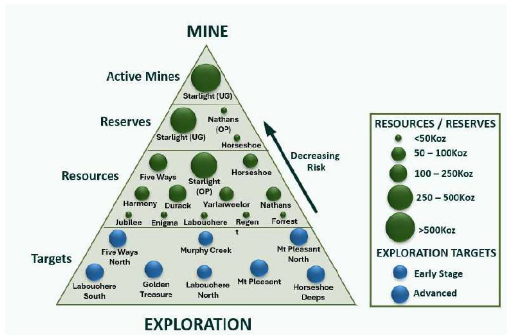
Figure 25-2 FGO Exploration Target Pipeline - Source: Westgold, 2025.
