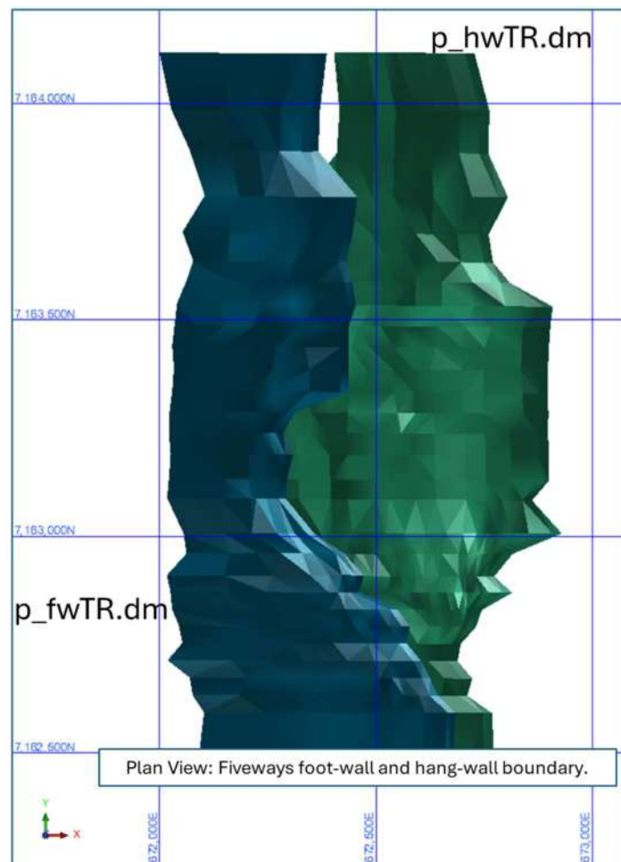
Figure 14-39 Fiveways mineralisation wireframes plan view. Source: Westgold.
