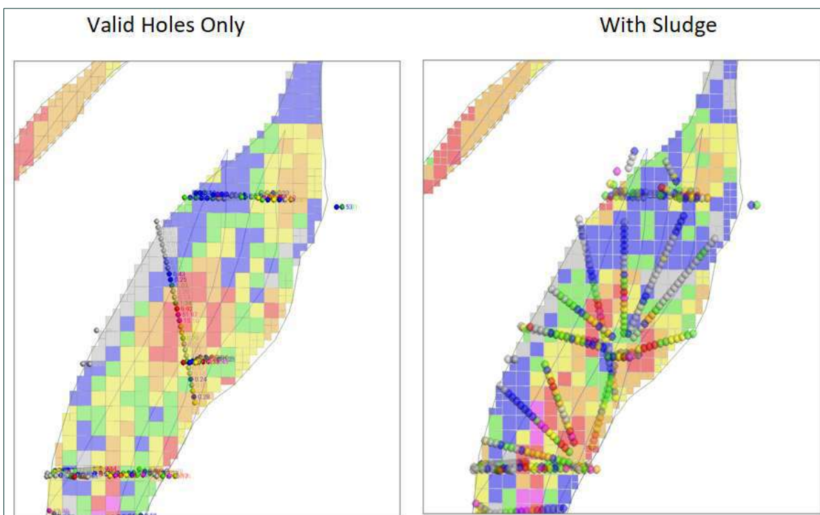
Figure 14-25 Section comparison showing estimate with and without sludge drilling - Source: Westgold.
