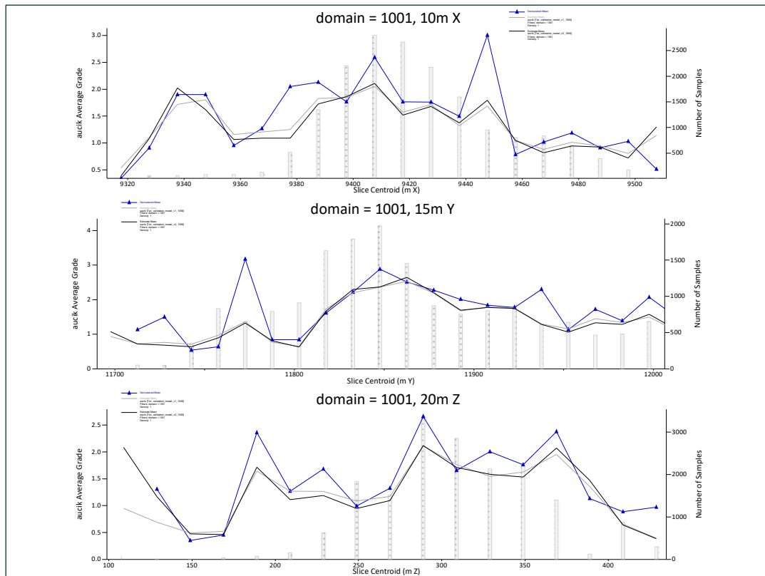
Figure 14-17 Domain 1001 validation swath plots - Source: Westgold.
