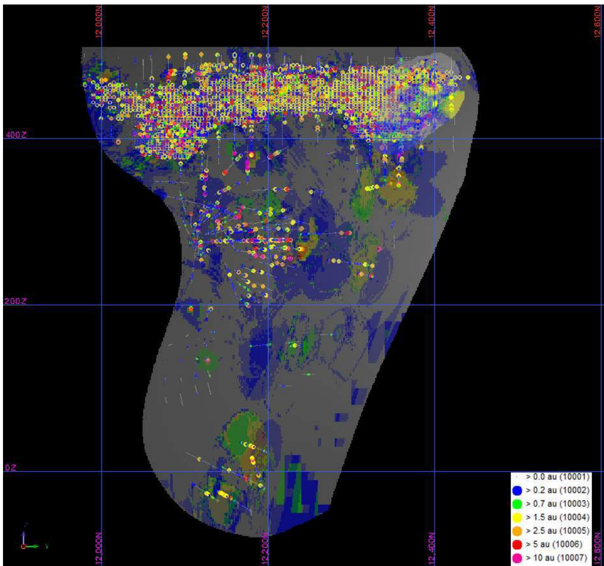
Figure 14-20 Domain 3000 - Dougie’s/Waterbore blocks versus composite data (coloured by au_final) – Note the large number of internal waste/LG blocks at depth informed by relatively few samples - Source: Westgold.
