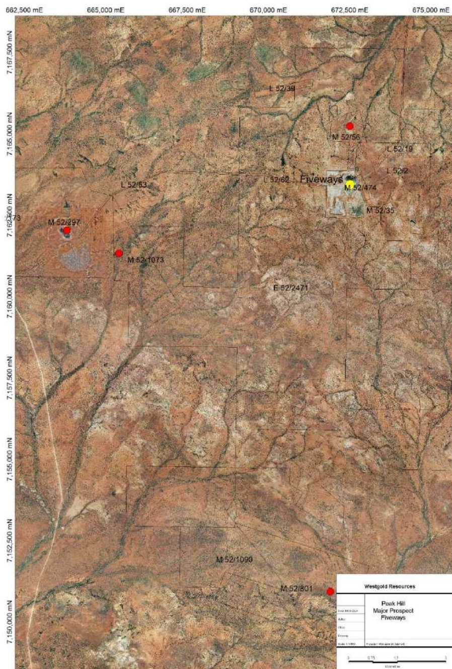
Figure 14-38 Fiveways deposit location map. Source: Westgold.
