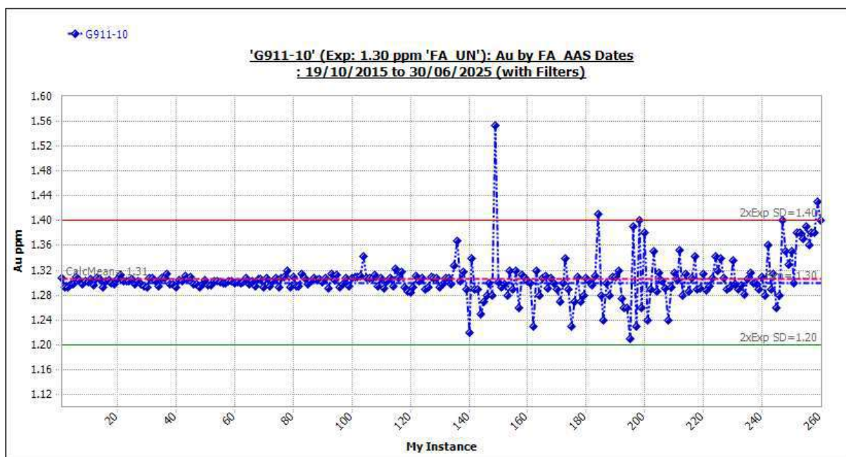
Figure 11-33 Standard G911-10: Outliers Included.
