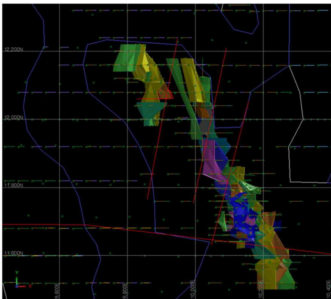
Figure 14-36 Geology of Enigma and Enigma West - note north-northeasterly (Baxter's grid) trending faults with apparent sinistral movement offsetting vein arrays. Source: Westgold.
