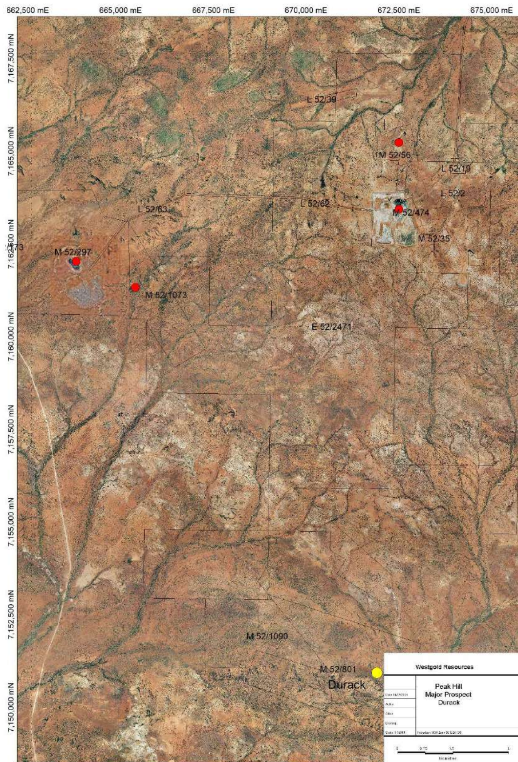
Figure 14-32 Durack deposit location map. Source: Westgold.
