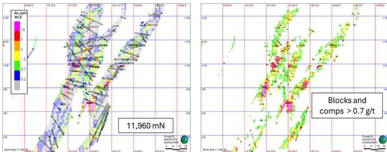
Figure 14-22 Cross section view at 11,960mN; Au ppm block grades versus gold assays – all samples (left) and above a 0.7 g/t (right) - Source: Westgold.
