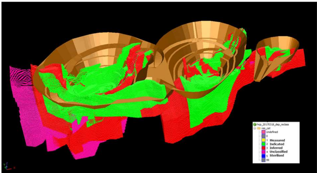
Figure 14-31 Classification scheme of the HCP Mineral Resource 2018 in relation to the current pit design files. Source: Westgold.
