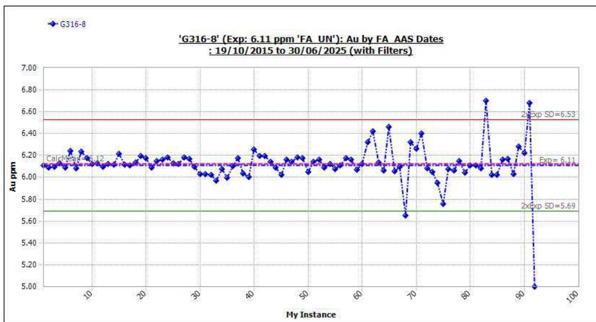
Figure 11-20 Standard G316-8: Outliers Included.
