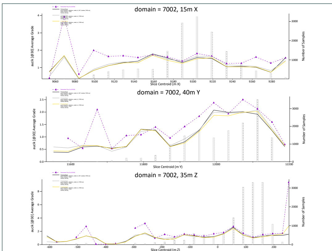
Figure 14-18 Domain 7002 validation swath plots - Source: Westgold.
