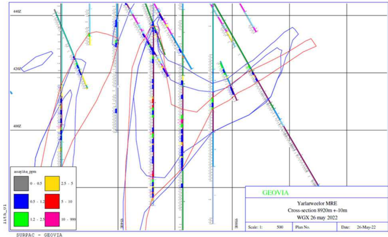
Figure 14-27 Cross-section at 8,920m northing showing the change in the domain interpretations between 2018 (blue) limited to the logged jasperoids and 2022 (red) limited to logged jasperoids and Au > 0.5 g/t; excluding external waste zones. Source: Westgold.
