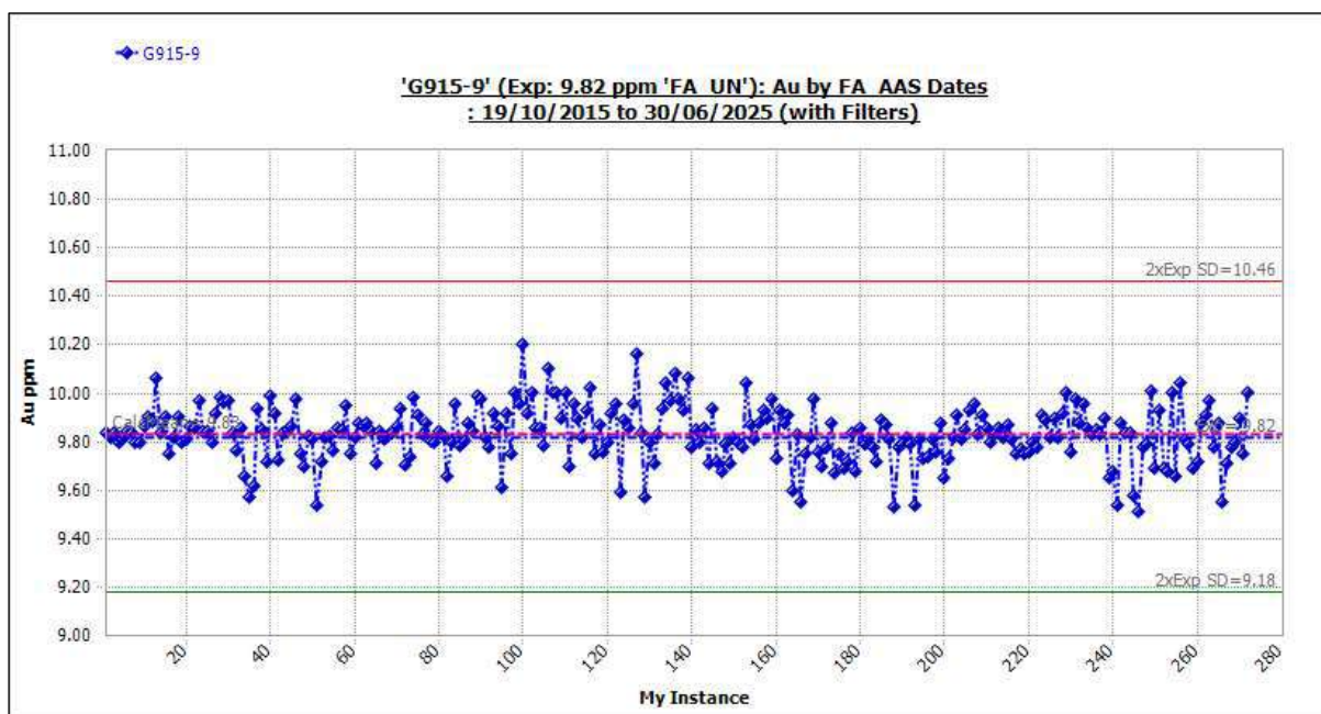
Figure 11-44 Standard G915-9: Outliers Included.
