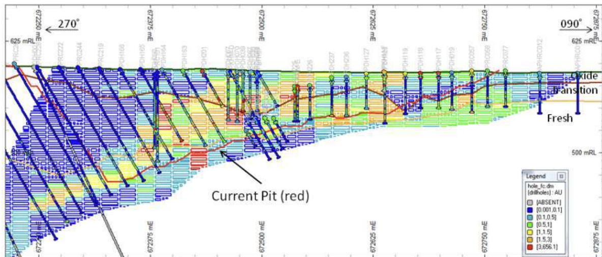
Figure 14-40 Visual comparison of gold grades at Fiveways between drillholes and estimated blocks. Source: Westgold.
