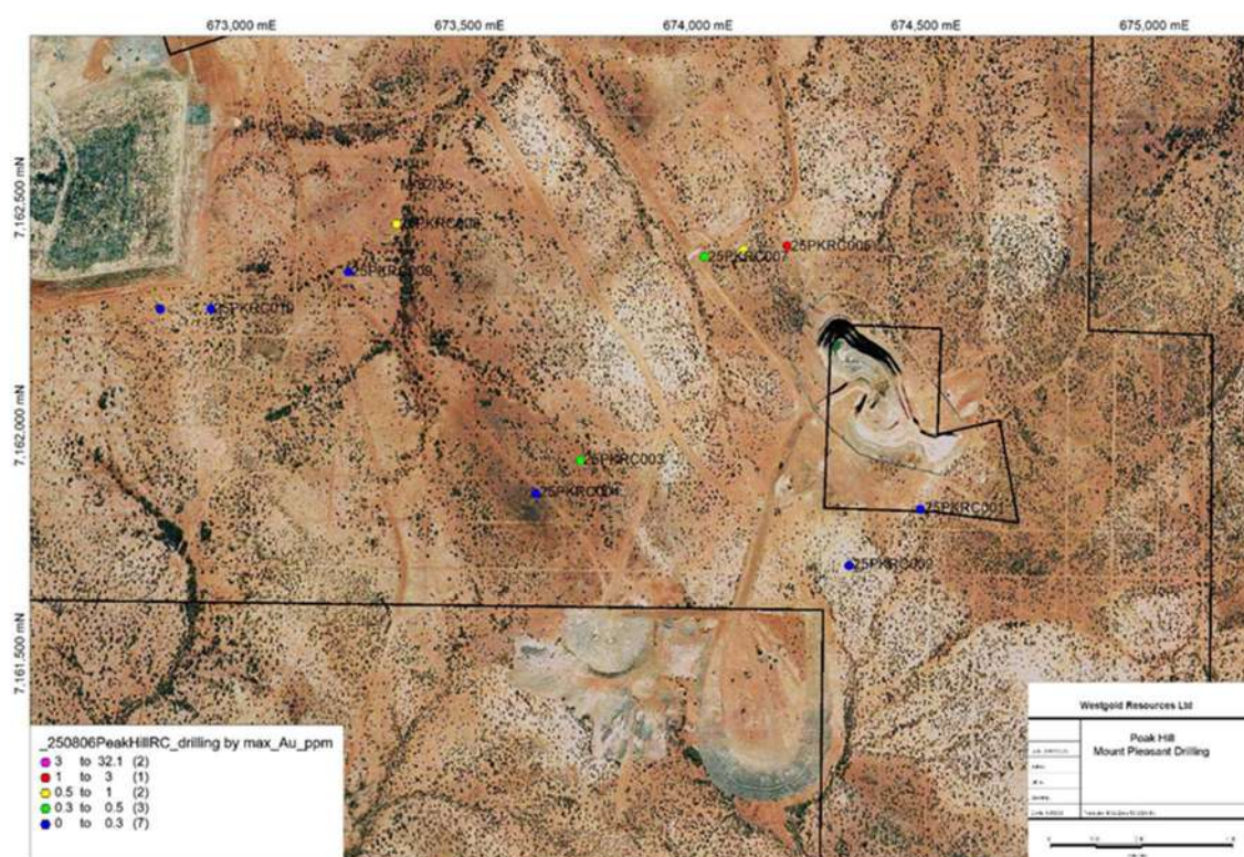
Figure 10-6 Mount Pleasant RC drill program - Source: Westgold.
