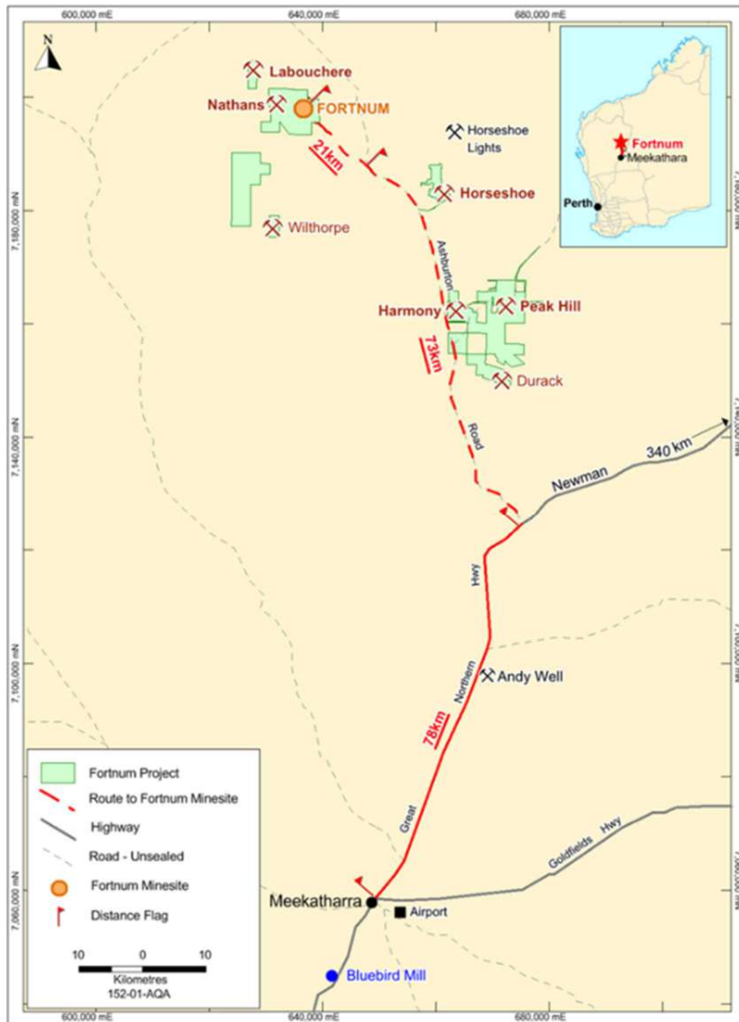
Figure 14-2 Location of deposits of the Fortnum Mineral Resources. Source: Westgold.
