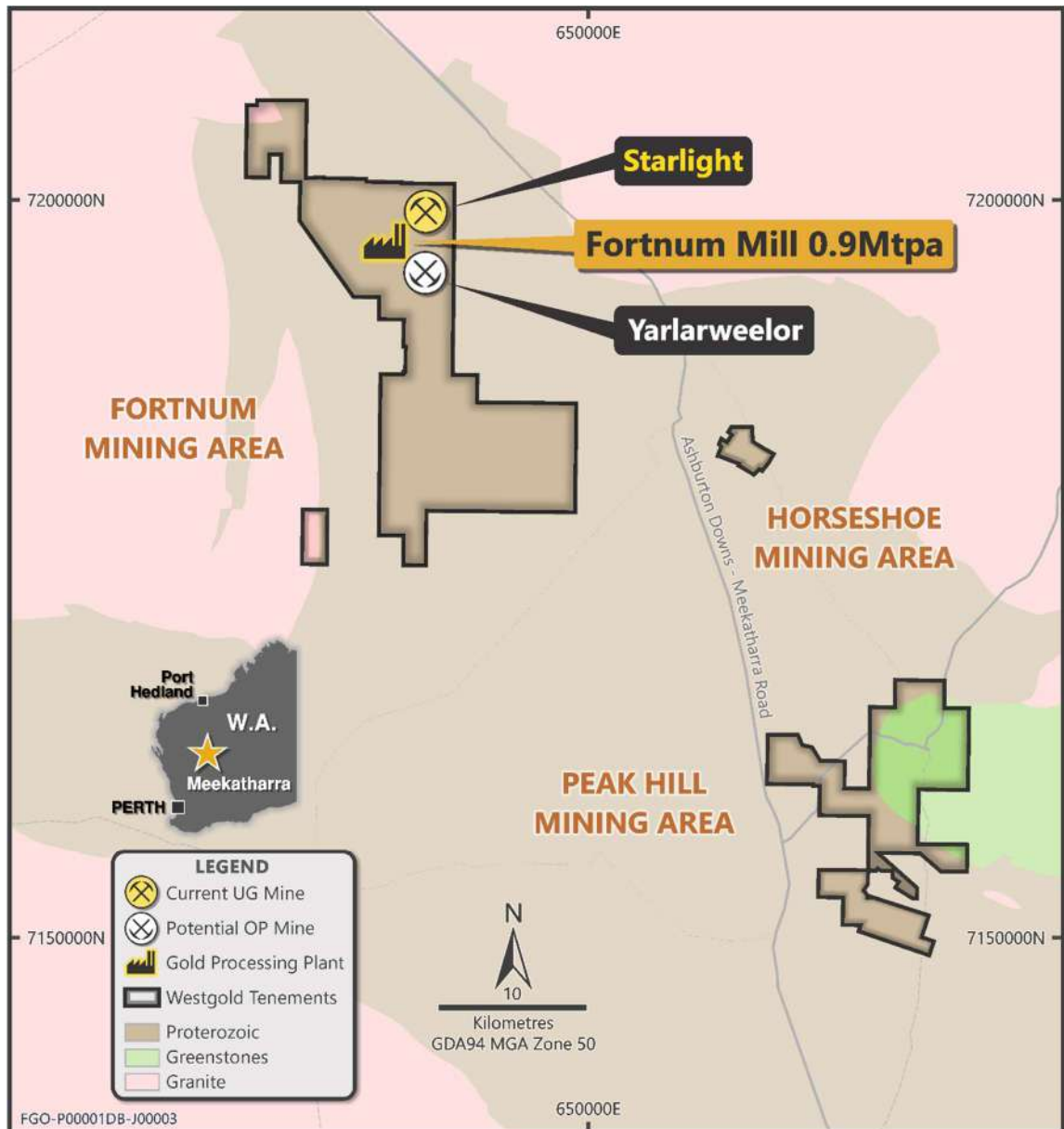
Figure 4-1 Westgold Bryah operations asset map - Source: Westgold.
