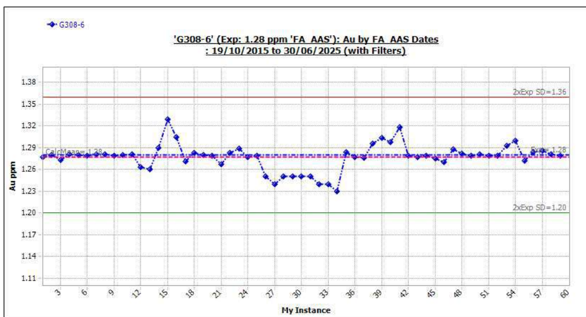
Figure 11-4 Standard G308-6: Outliers Included.
