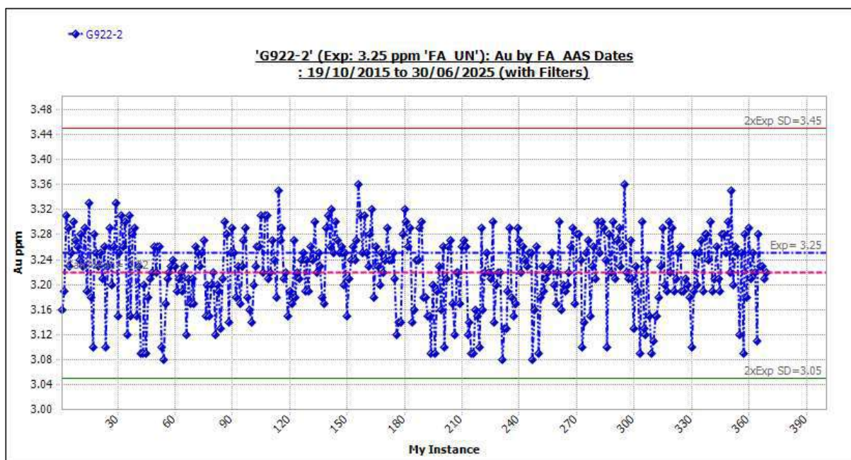
Figure 11-51 Standard G922-2: Outliers Included.
