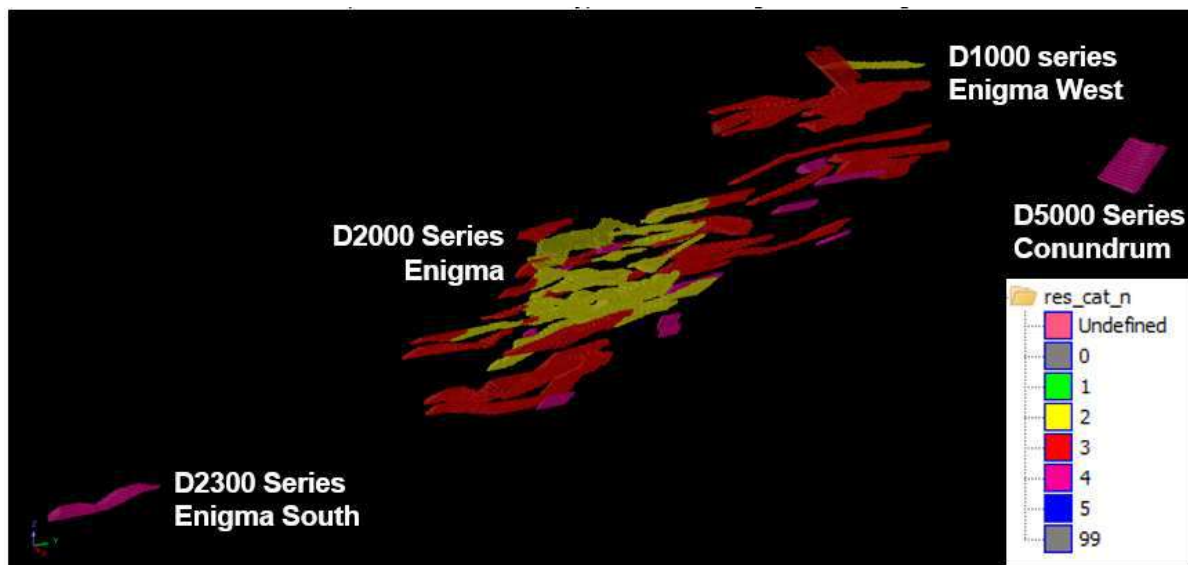
Figure 14-37 Classification of Enigma Mineral Resource Estimate. Viewed from above, looking northwest. Source: Westgold.
