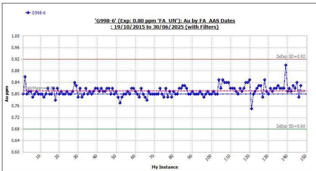
Figure 11-53 Standard G998-6: Outliers Included.
