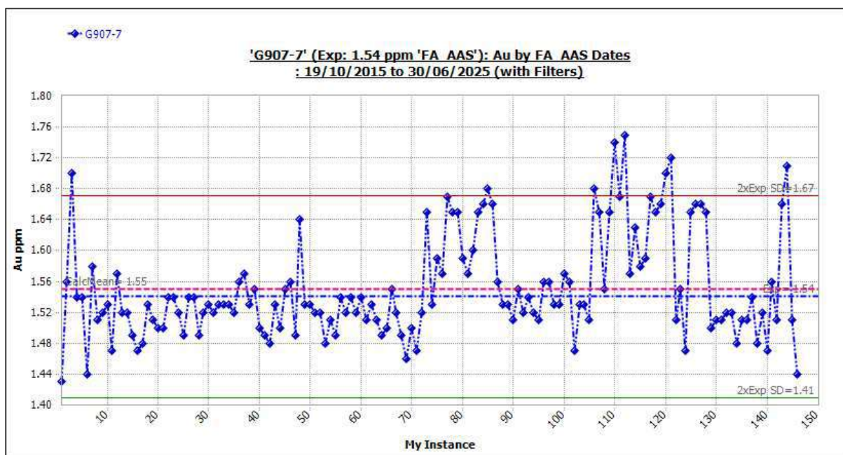
Figure 11-32 Standard G907-7: Outliers Included.
