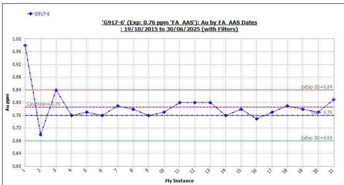
Figure 11-49 Standard G917-6: Outliers Included.
