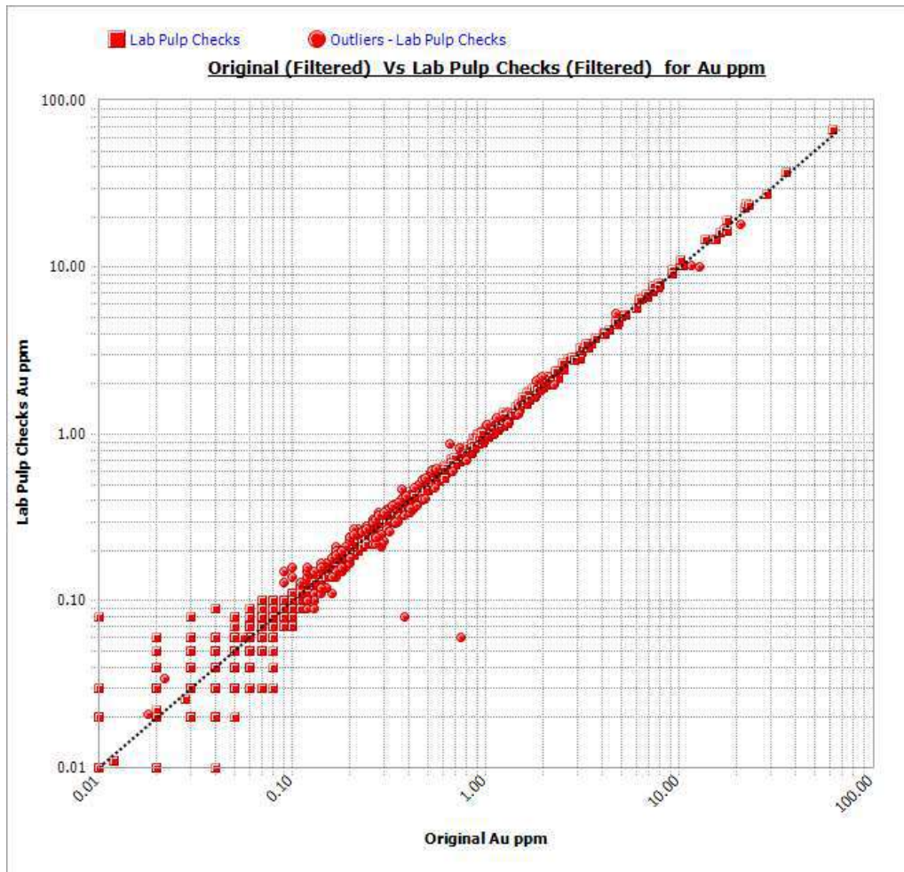
Figure 11-56 Q-Q Plot - drillhole (Repeat Code) : original v. laboratory pulp checks for Au ppm.
