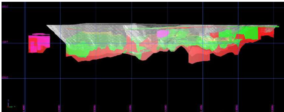
Figure 14-28 Resource Classification of Yarlarweelor (Yellow = Measured, Green = Indicated, Red = Inferred, Magenta = Unclassified, White = A$2,000 optimised pit shell). Depleted material removed and looking northwest with minor plunge. (a) looking northwest; and, (b) long section view. Source: Westgold.
