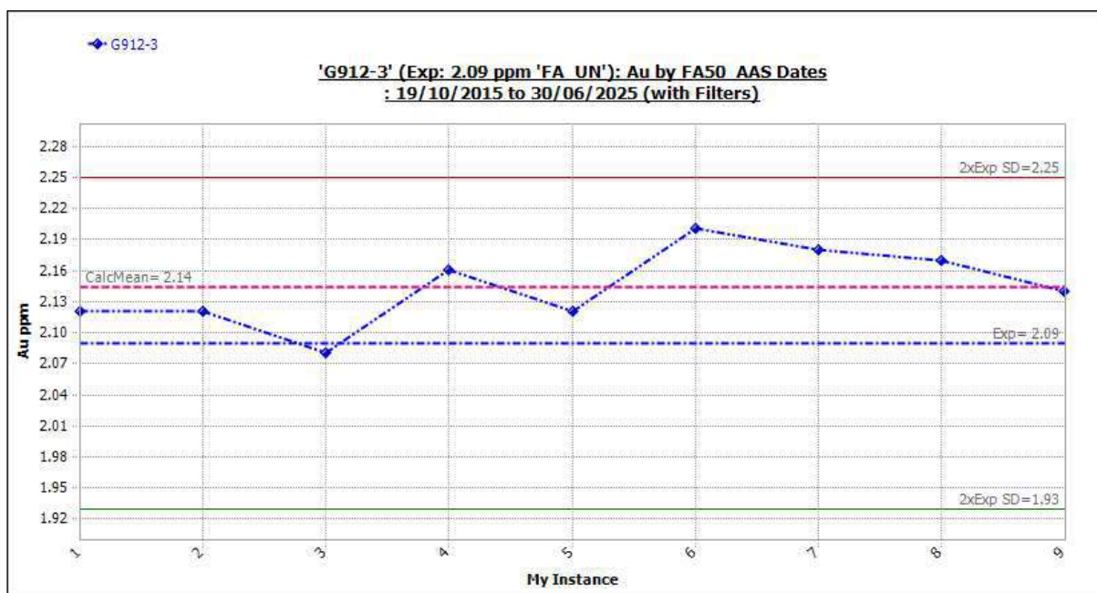
Figure 11-35 Standard G912-3: Outliers Included.
