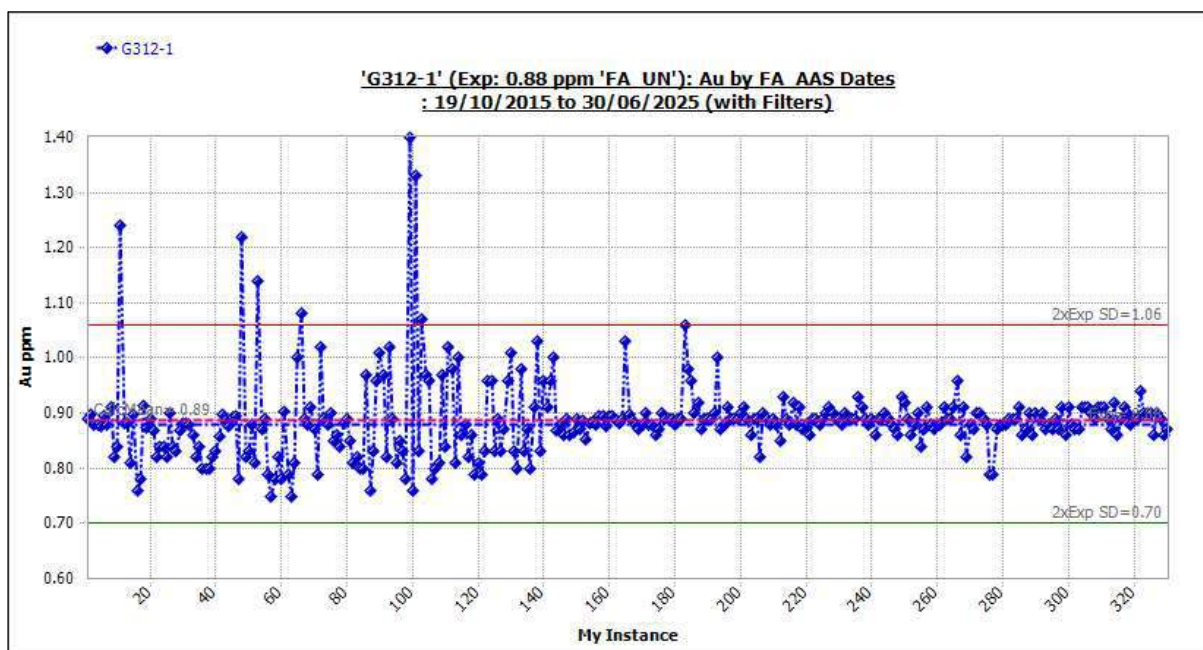
Figure 11-7 Standard G312-1: Outliers Included.
