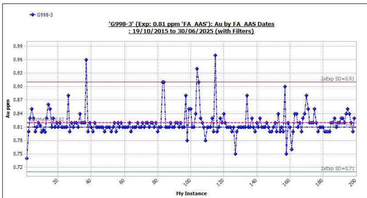
Figure 11-52 Standard G998-3: Outliers Included.
