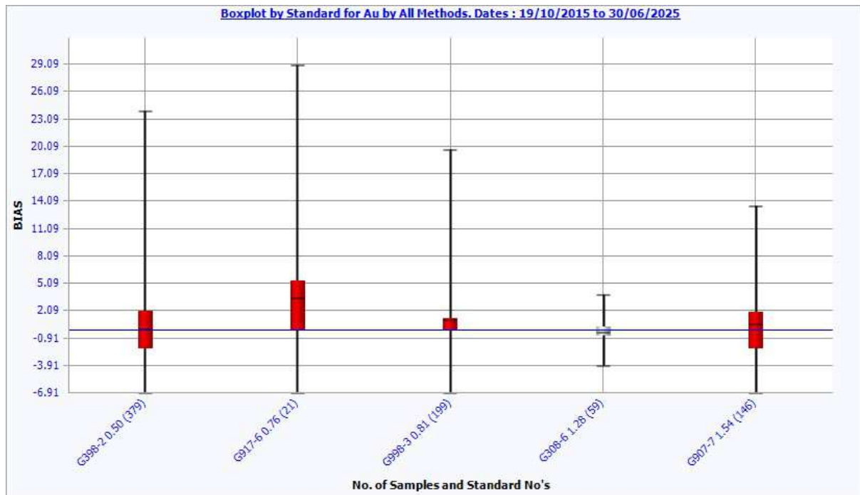
Figure 11-58 Boxplot by Standard for Au by all methods.
