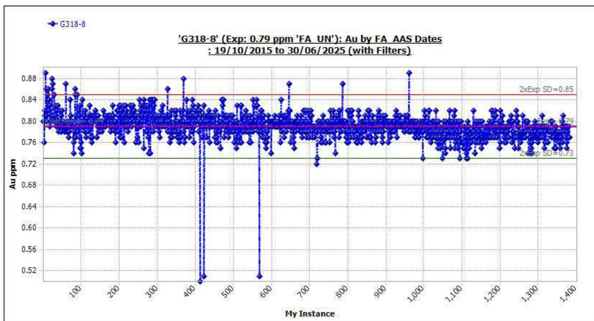
Figure 11-23 Standard G318-8: Outliers Included.
