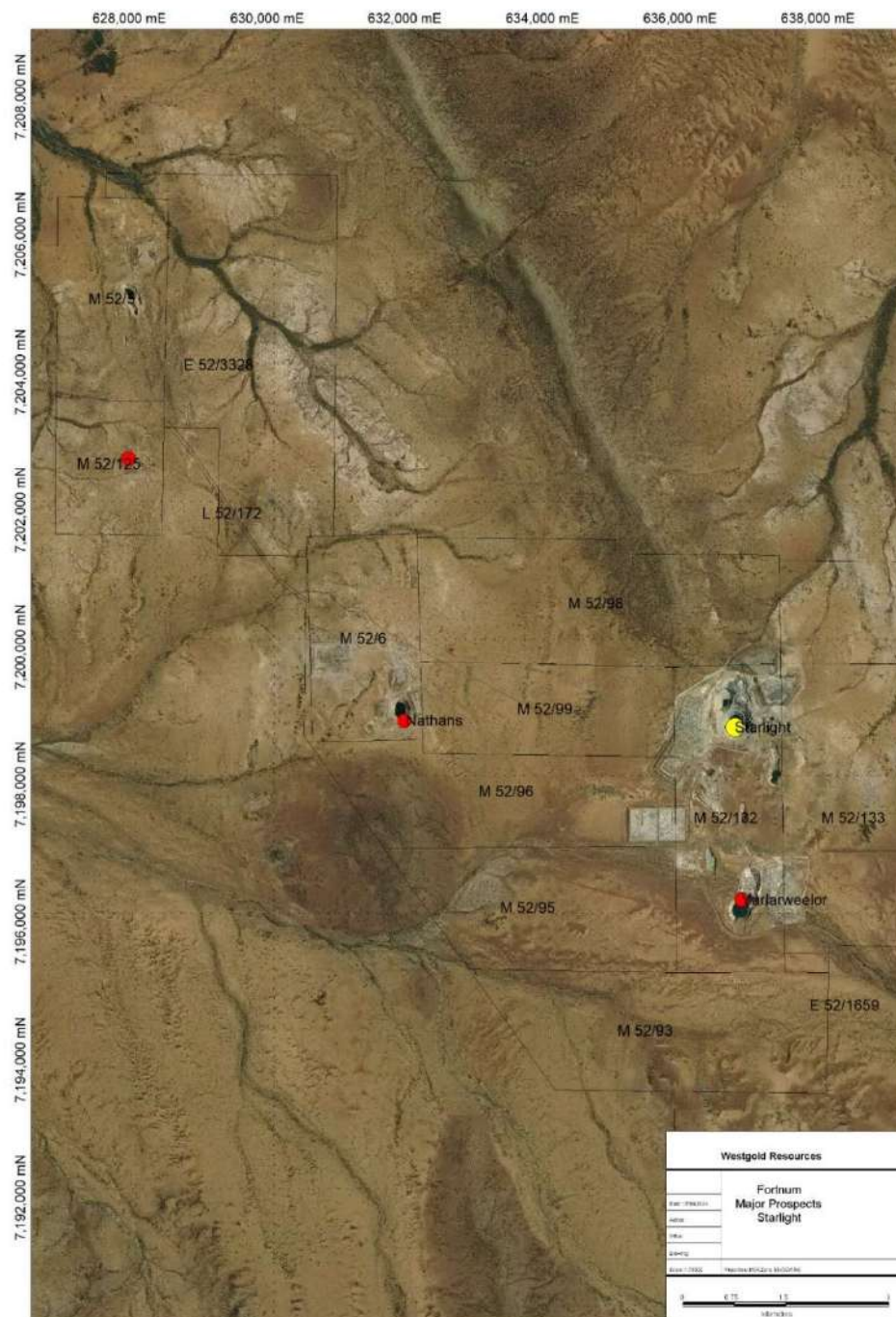
Figure 14-13 Starlight deposit location map - Source: Westgold.
