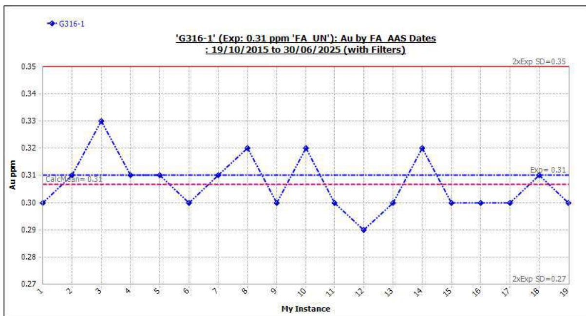
Figure 11-17 Standard G316-1: Outliers Included.
