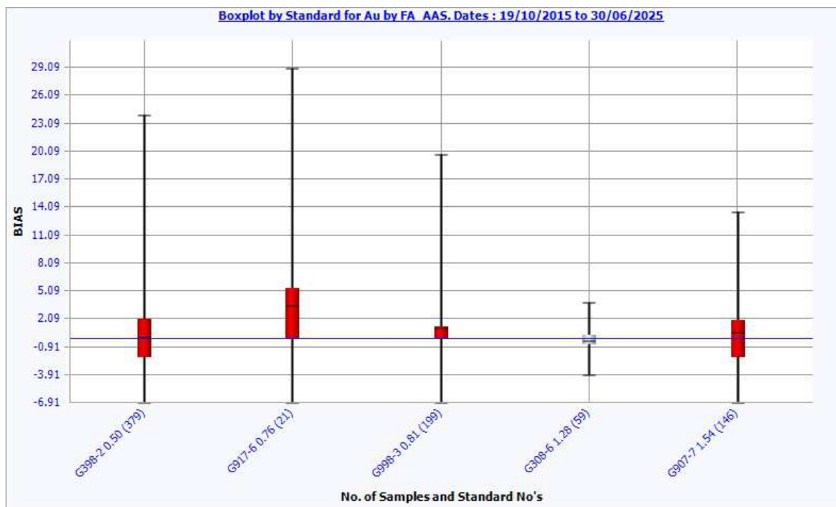
Figure 11-59 Boxplot by Standard for Au by Fire Assay AAS.
