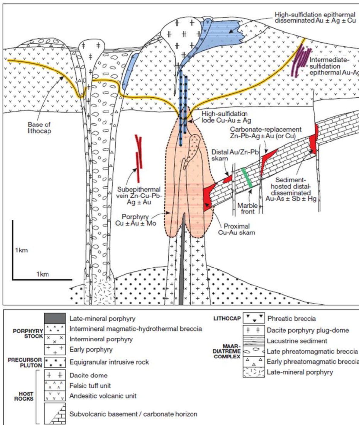
Figure 8-1: Schematic Model
