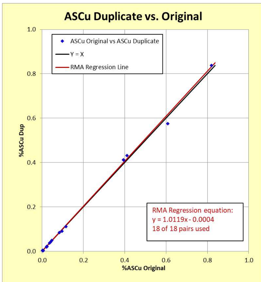
Figure 11-23: 2023 Crush-Duplicate Acid-Soluble Copper (“ASCu”) Results Relative to Primary Sample Assays
