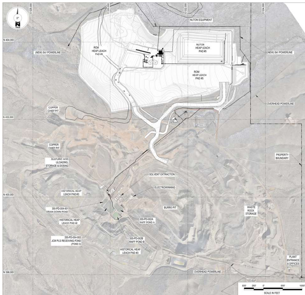
Figure 1-2: Site Plan of the Johnson Camp Mine showing the location of new leach pad, Pad 5
